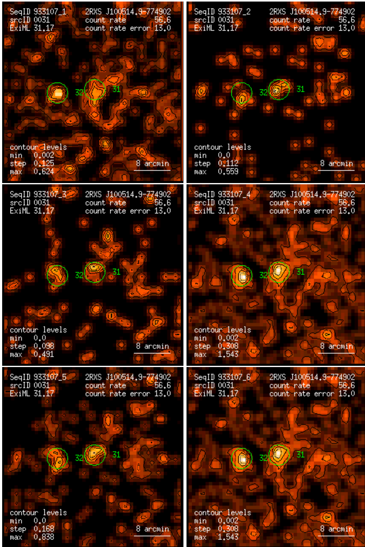
Figure 31: RASS 933107: detection 0031: band rate images, Gaussian filter: (1) PSPC channels 11 – 41, (2) 52 – 90, (3) 91 – 201, (4) 11 – 235, (5) 52 – 201, (6) 11 – 201. Broad band rates in counts/ks. Band rate contour levels in counts/ks/arcmin 2 .
