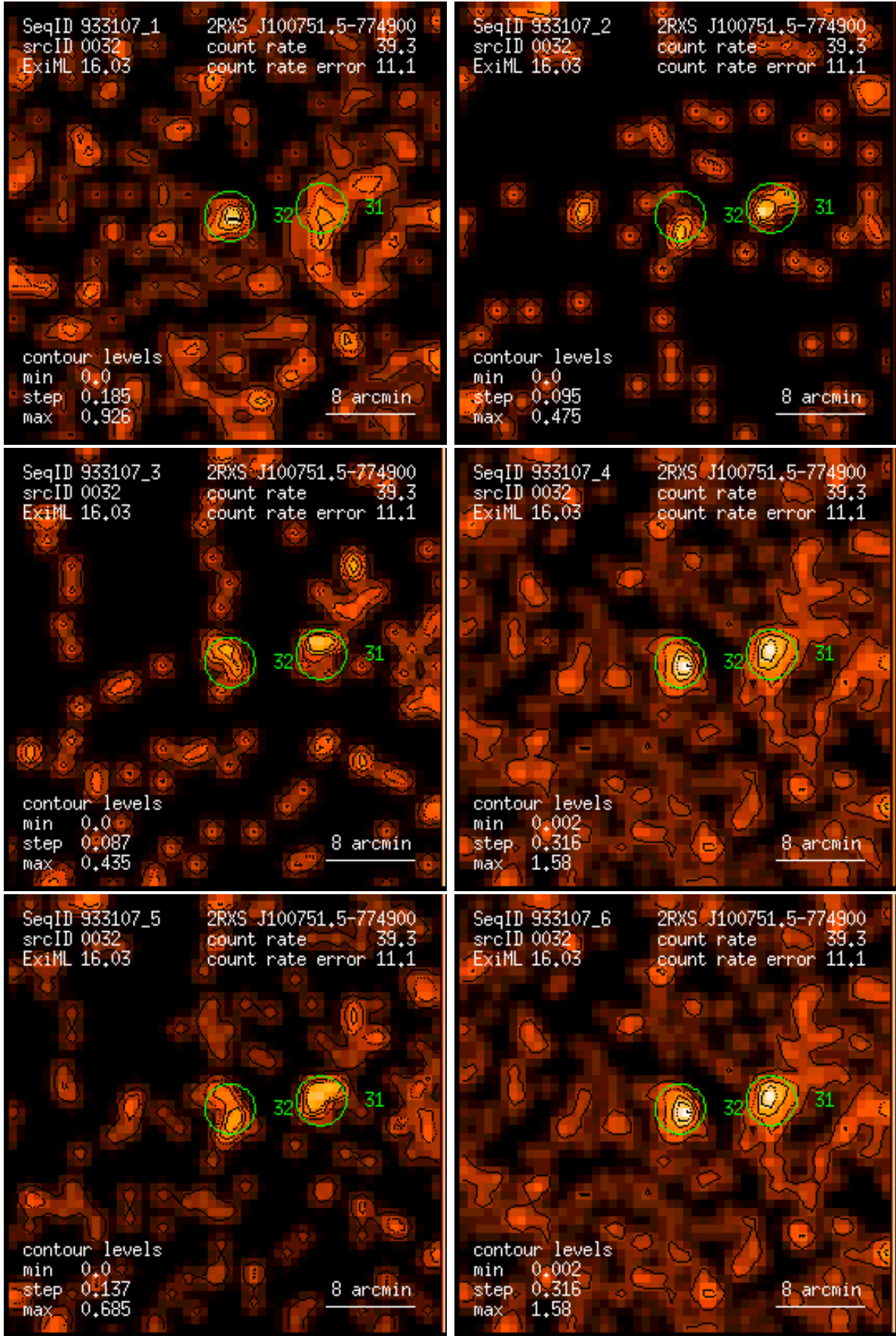
Figure 32: RASS 933107: detection 0032: band rate images, Gaussian filter: (1) PSPC channels 11 – 41, (2) 52 – 90, (3) 91 – 201, (4) 11 – 235, (5) 52 – 201, (6) 11 – 201. Broad band rates in counts/ks. Band rate contour levels in counts/ks/arcmin 2 .
