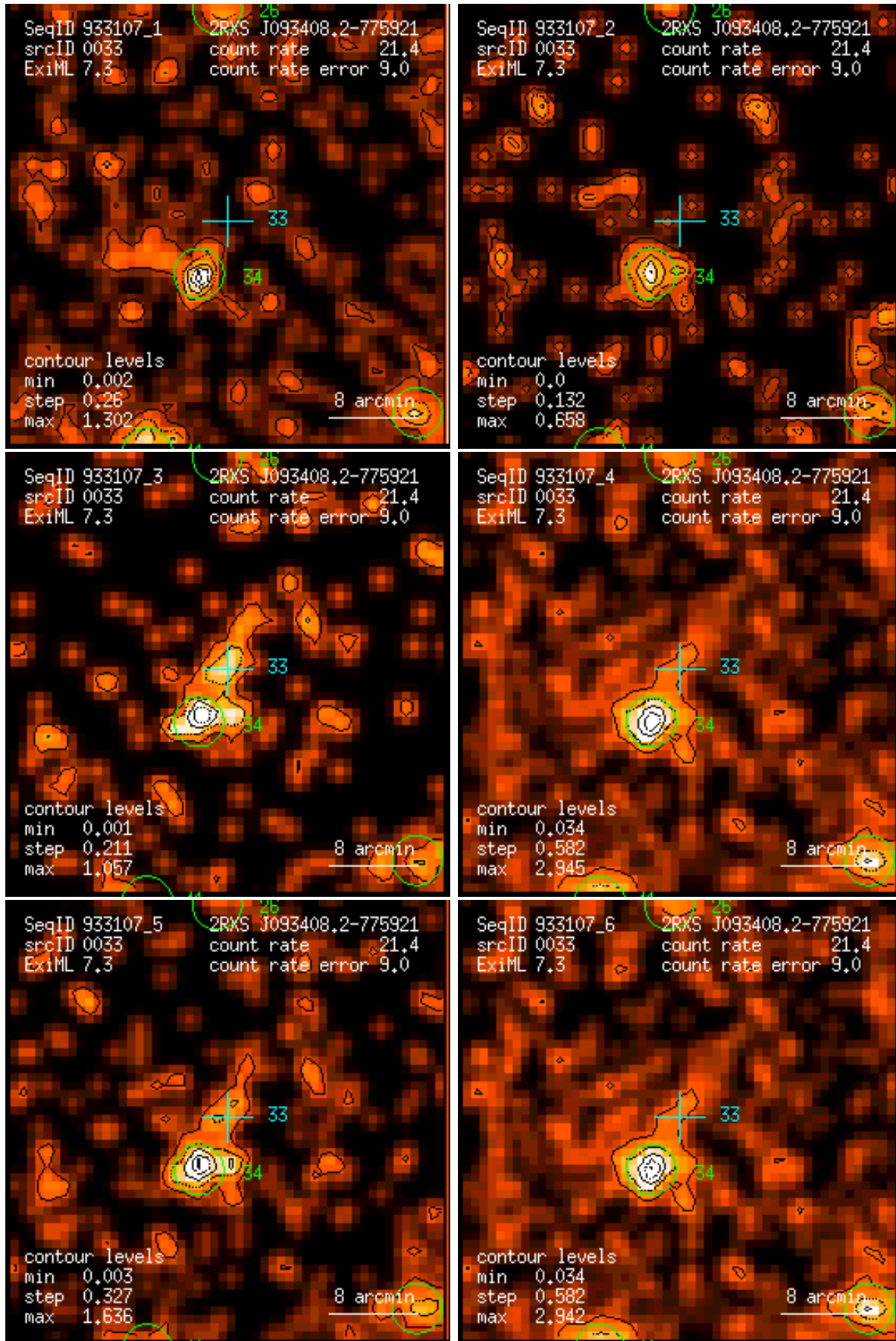
Figure 33: RASS 933107: detection 0033: band rate images, Gaussian filter: (1) PSPC channels 11 – 41, (2) 52 – 90, (3) 91 – 201, (4) 11 – 235, (5) 52 – 201, (6) 11 – 201. Broad band rates in counts/ks. Band rate contour levels in counts/ks/arcmin 2 .
