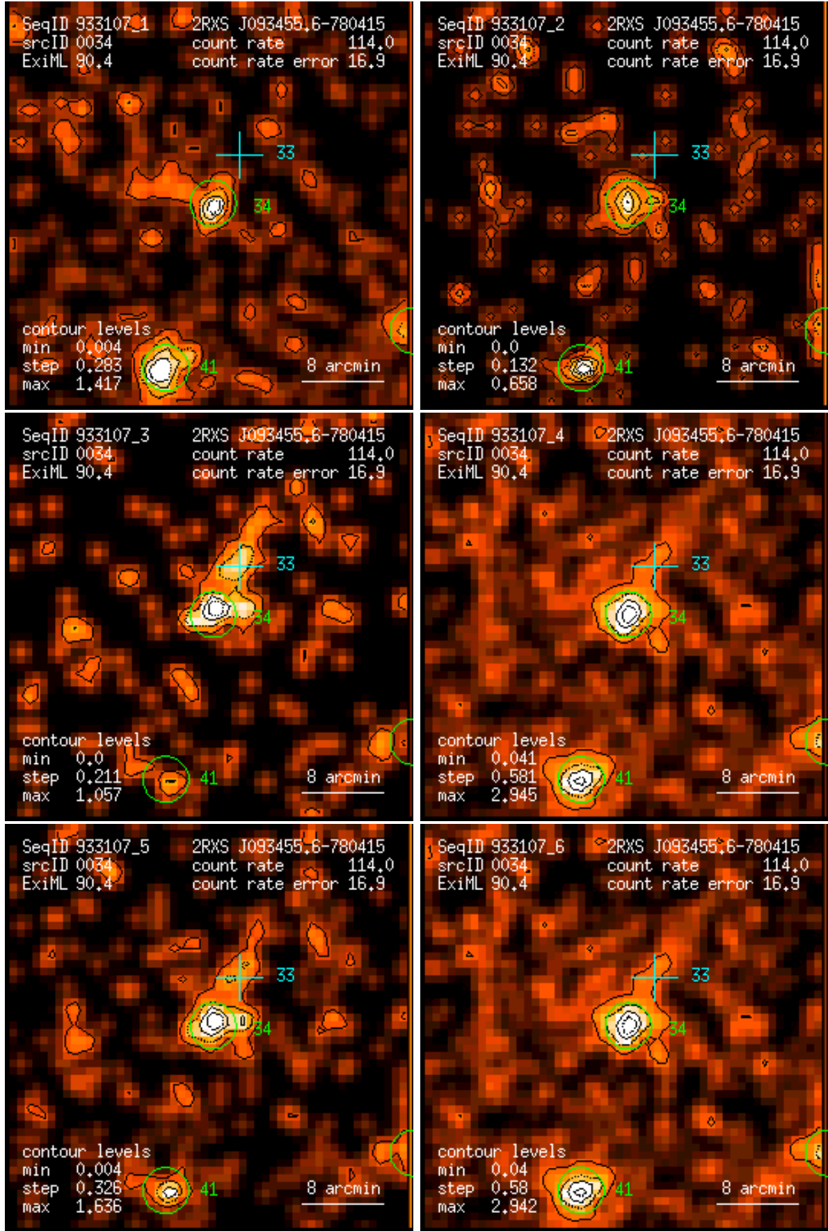
Figure 34: RASS 933107: detection 0034: band rate images, Gaussian filter: (1) PSPC channels 11 – 41, (2) 52 – 90, (3) 91 – 201, (4) 11 – 235, (5) 52 – 201, (6) 11 – 201. Broad band rates in counts/ks. Band rate contour levels in counts/ks/arcmin 2 .
