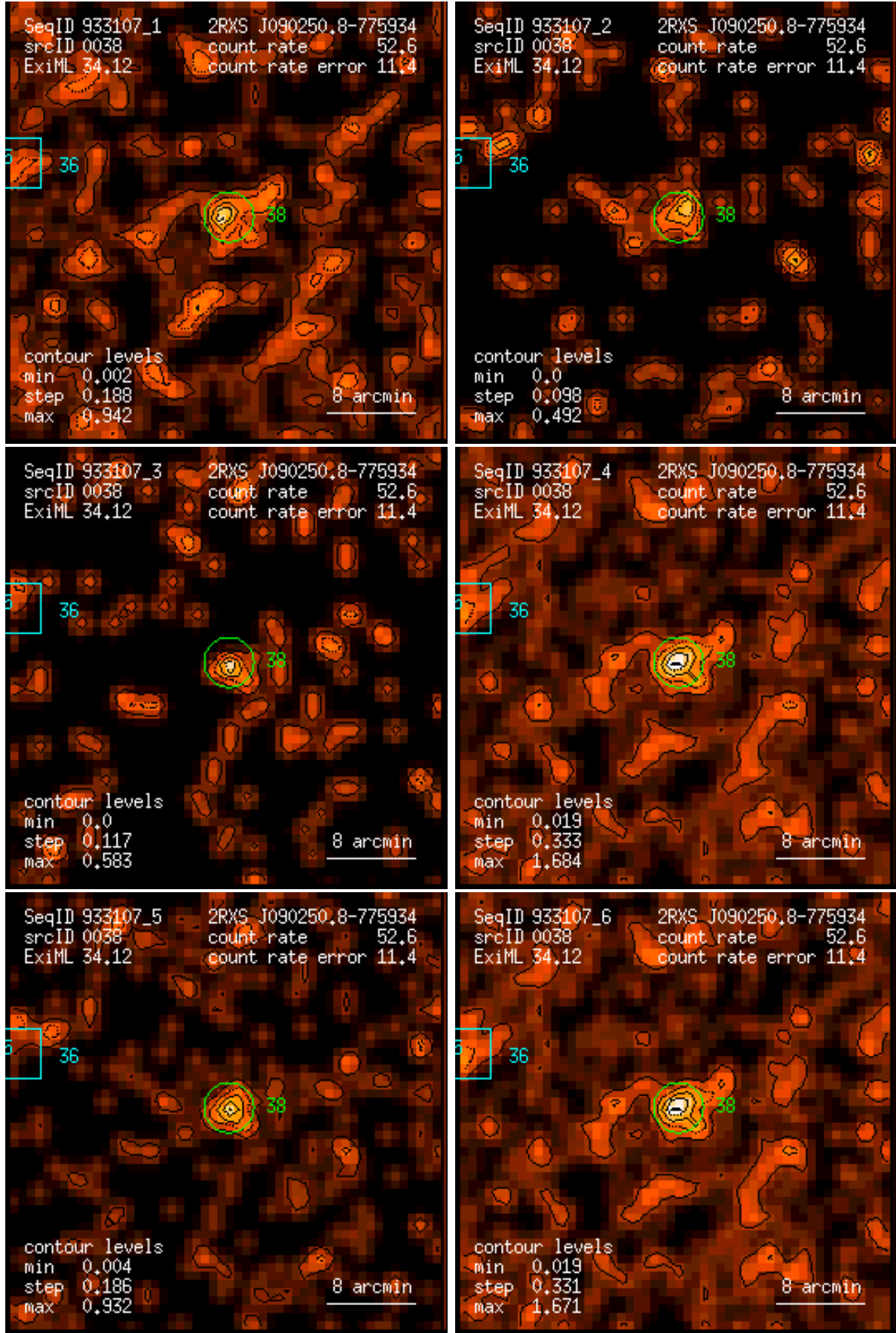
Figure 38: RASS 933107: detection 0038: band rate images, Gaussian filter: (1) PSPC channels 11 – 41, (2) 52 – 90, (3) 91 – 201, (4) 11 – 235, (5) 52 – 201, (6) 11 – 201. Broad band rates in counts/ks. Band rate contour levels in counts/ks/arcmin 2 .
