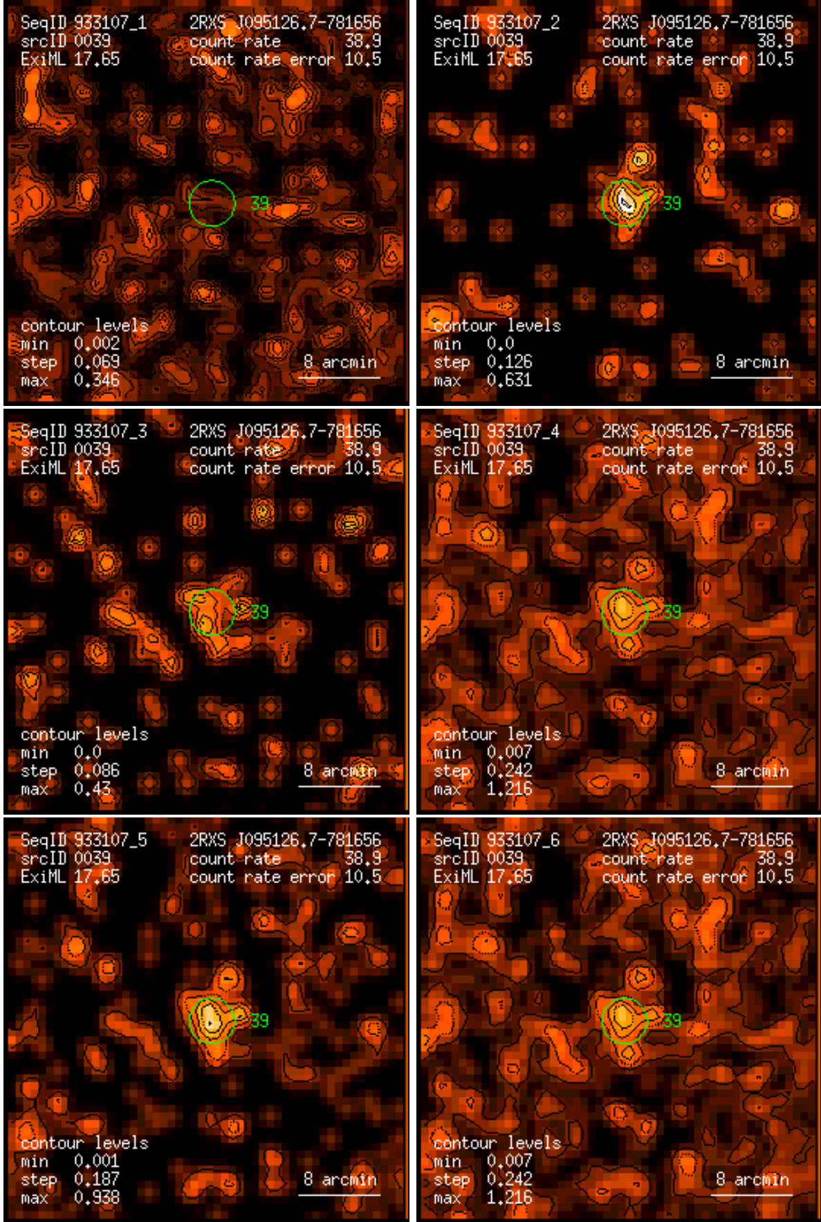
Figure 39: RASS 933107: detection 0039: band rate images, Gaussian filter: (1) PSPC channels 11 – 41, (2) 52 – 90, (3) 91 – 201, (4) 11 – 235, (5) 52 – 201, (6) 11 – 201. Broad band rates in counts/ks. Band rate contour levels in counts/ks/arcmin 2 .
