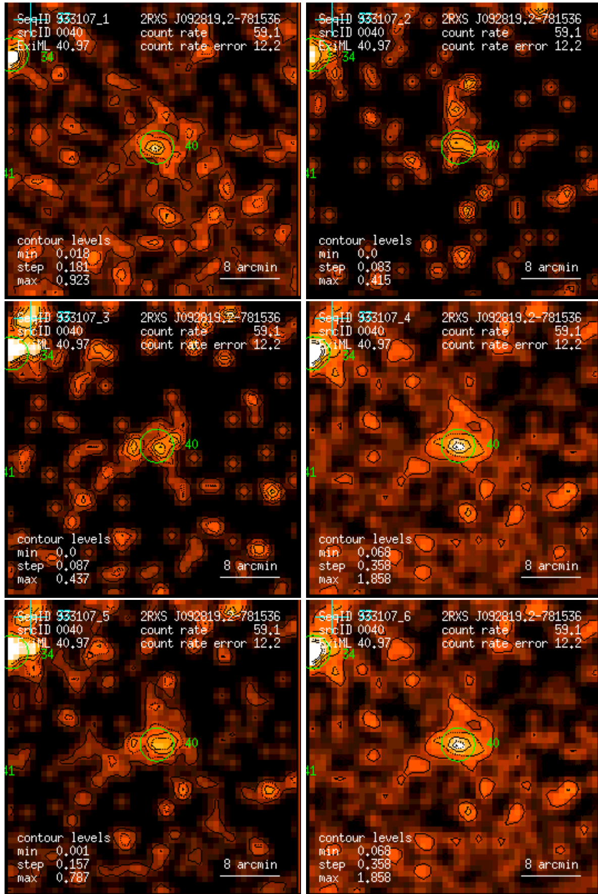
Figure 40: RASS 933107: detection 0040: band rate images, Gaussian filter: (1) PSPC channels 11 – 41, (2) 52 – 90, (3) 91 – 201, (4) 11 – 235, (5) 52 – 201, (6) 11 – 201. Broad band rates in counts/ks. Band rate contour levels in counts/ks/arcmin 2 .
