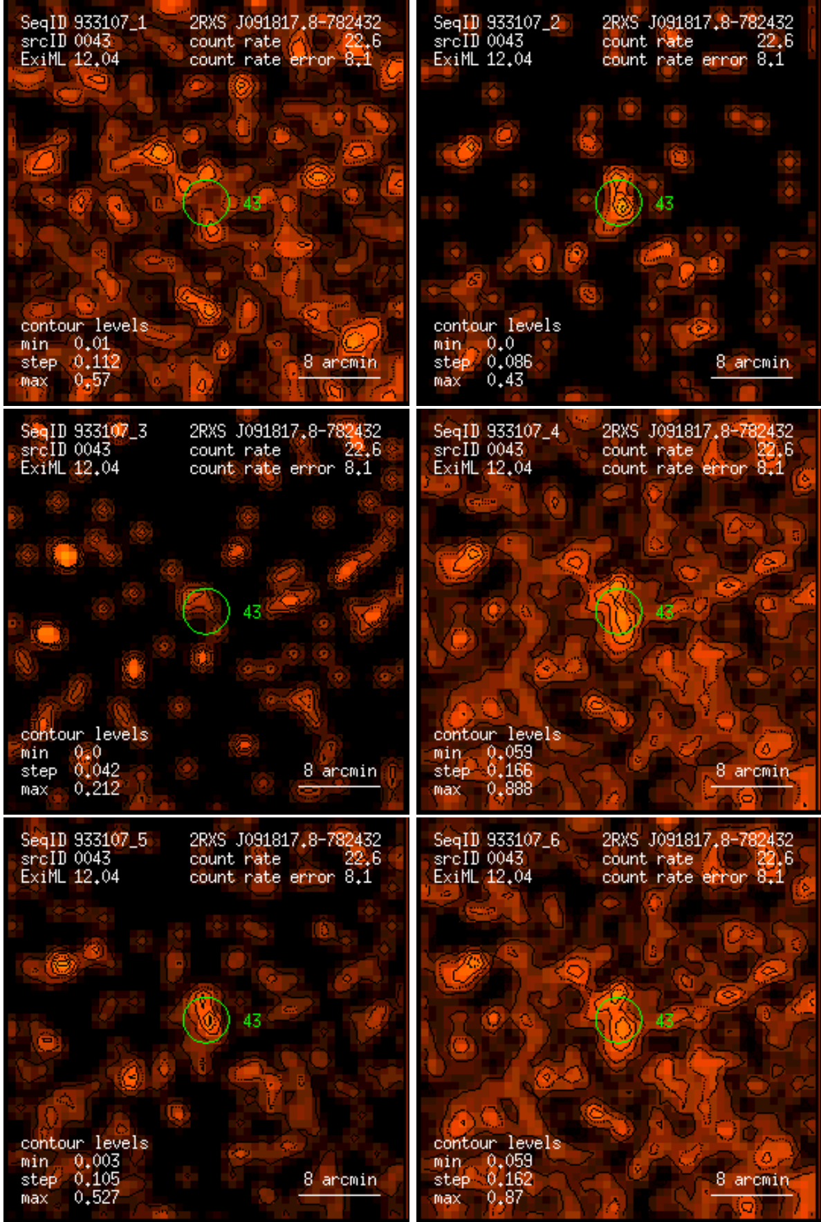
Figure 43: RASS 933107: detection 0043: band rate images, Gaussian filter: (1) PSPC channels 11 – 41, (2) 52 – 90, (3) 91 – 201, (4) 11 – 235, (5) 52 – 201, (6) 11 – 201. Broad band rates in counts/ks. Band rate contour levels in counts/ks/arcmin 2 .
