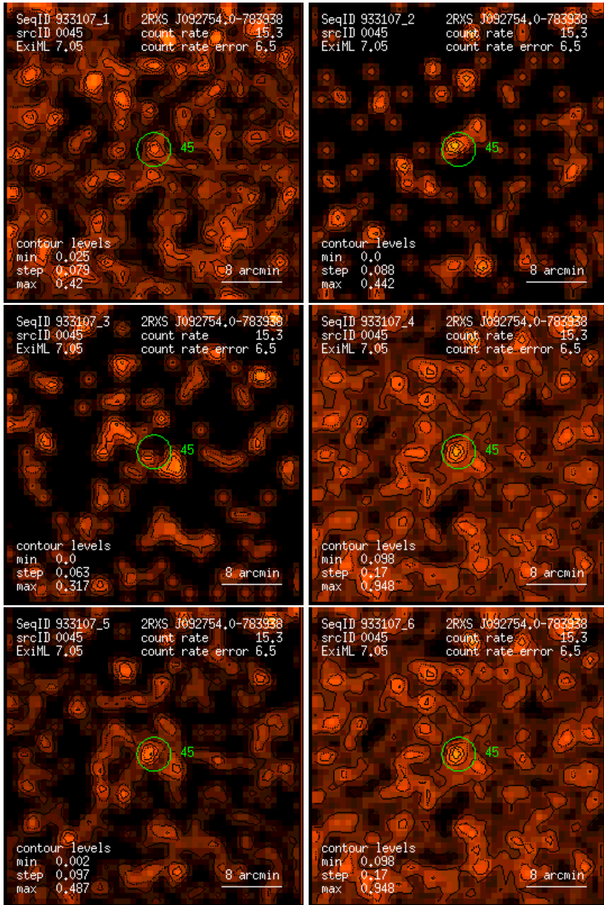
Figure 45: RASS 933107: detection 0045: band rate images, Gaussian filter: (1) PSPC channels 11 – 41, (2) 52 – 90, (3) 91 – 201, (4) 11 – 235, (5) 52 – 201, (6) 11 – 201. Broad band rates in counts/ks. Band rate contour levels in counts/ks/arcmin 2 .
