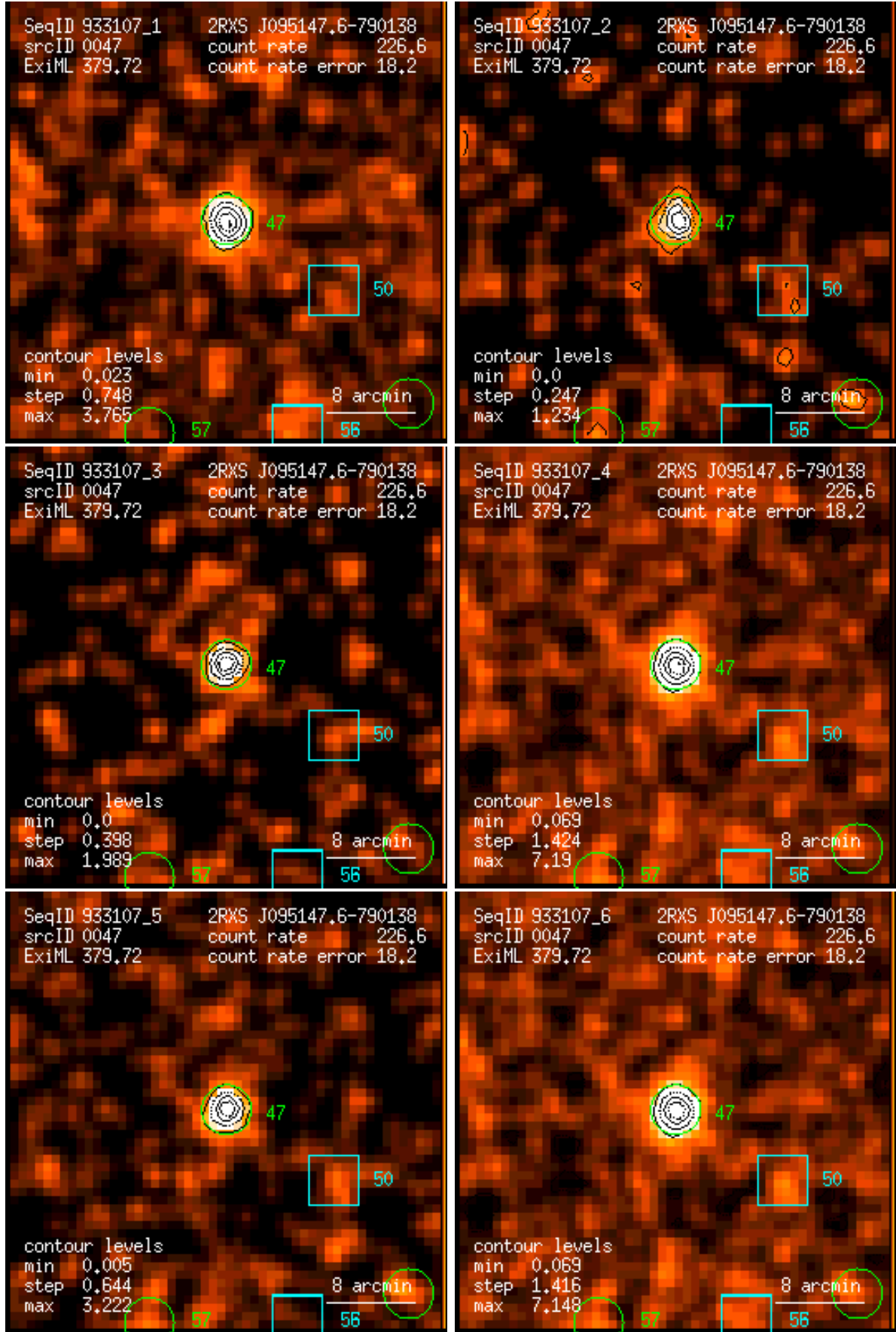
Figure 47: RASS 933107: detection 0047: band rate images, Gaussian filter: (1) PSPC channels 11 – 41, (2) 52 – 90, (3) 91 – 201, (4) 11 – 235, (5) 52 – 201, (6) 11 – 201. Broad band rates in counts/ks. Band rate contour levels in counts/ks/arcmin 2 .
