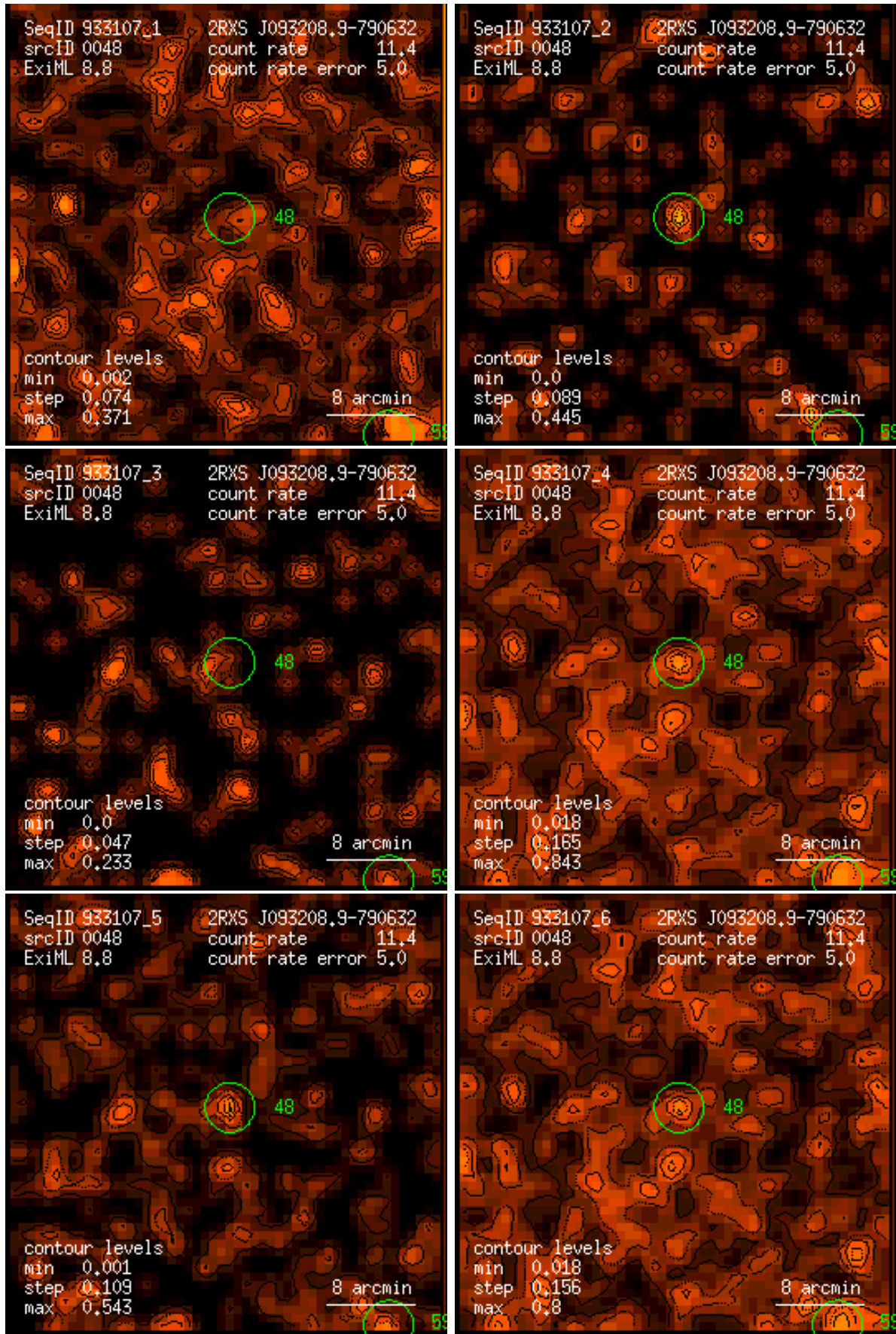
Figure 48: RASS 933107: detection 0048: band rate images, Gaussian filter: (1) PSPC channels 11 – 41, (2) 52 – 90, (3) 91 – 201, (4) 11 – 235, (5) 52 – 201, (6) 11 – 201. Broad band rates in counts/ks. Band rate contour levels in counts/ks/arcmin 2 .
