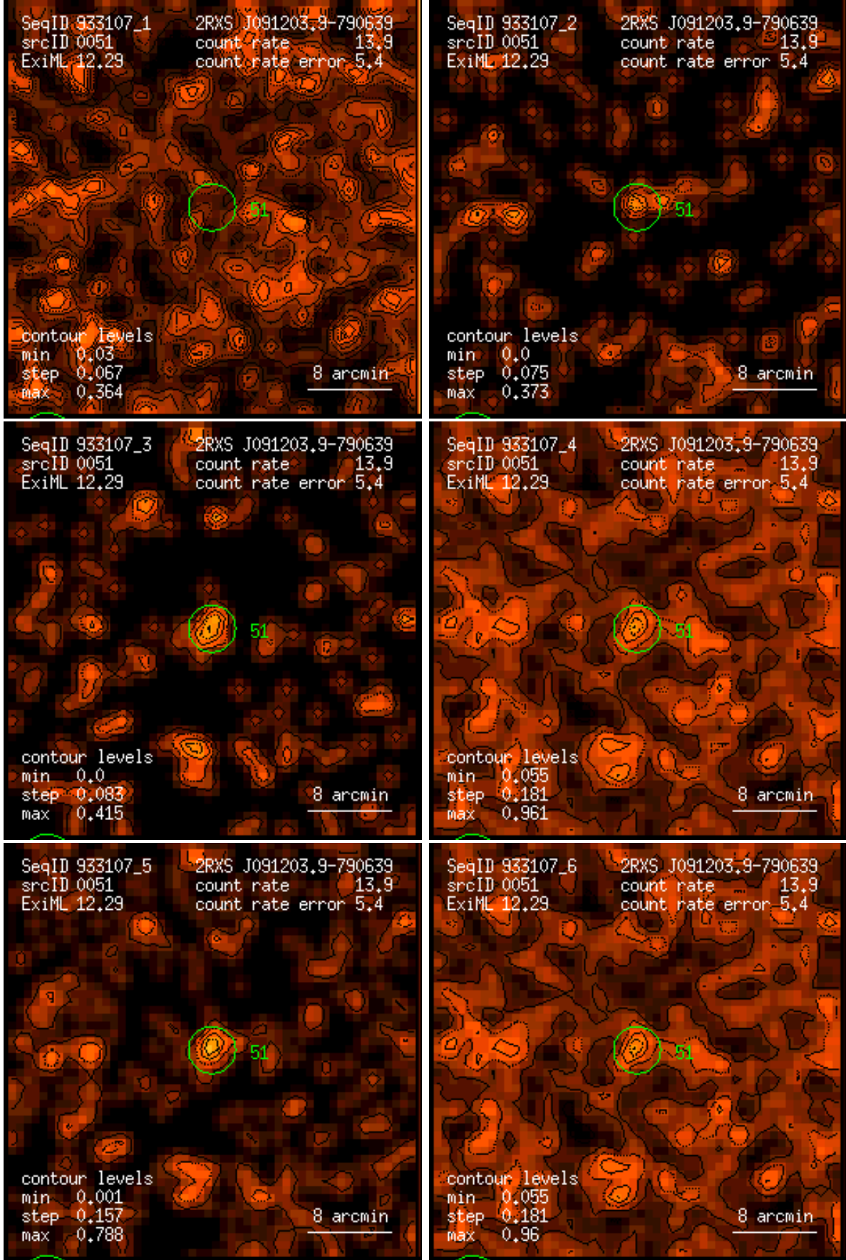
Figure 51: RASS 933107: detection 0051: band rate images, Gaussian filter: (1) PSPC channels 11 – 41, (2) 52 – 90, (3) 91 – 201, (4) 11 – 235, (5) 52 – 201, (6) 11 – 201. Broad band rates in counts/ks. Band rate contour levels in counts/ks/arcmin 2 .
