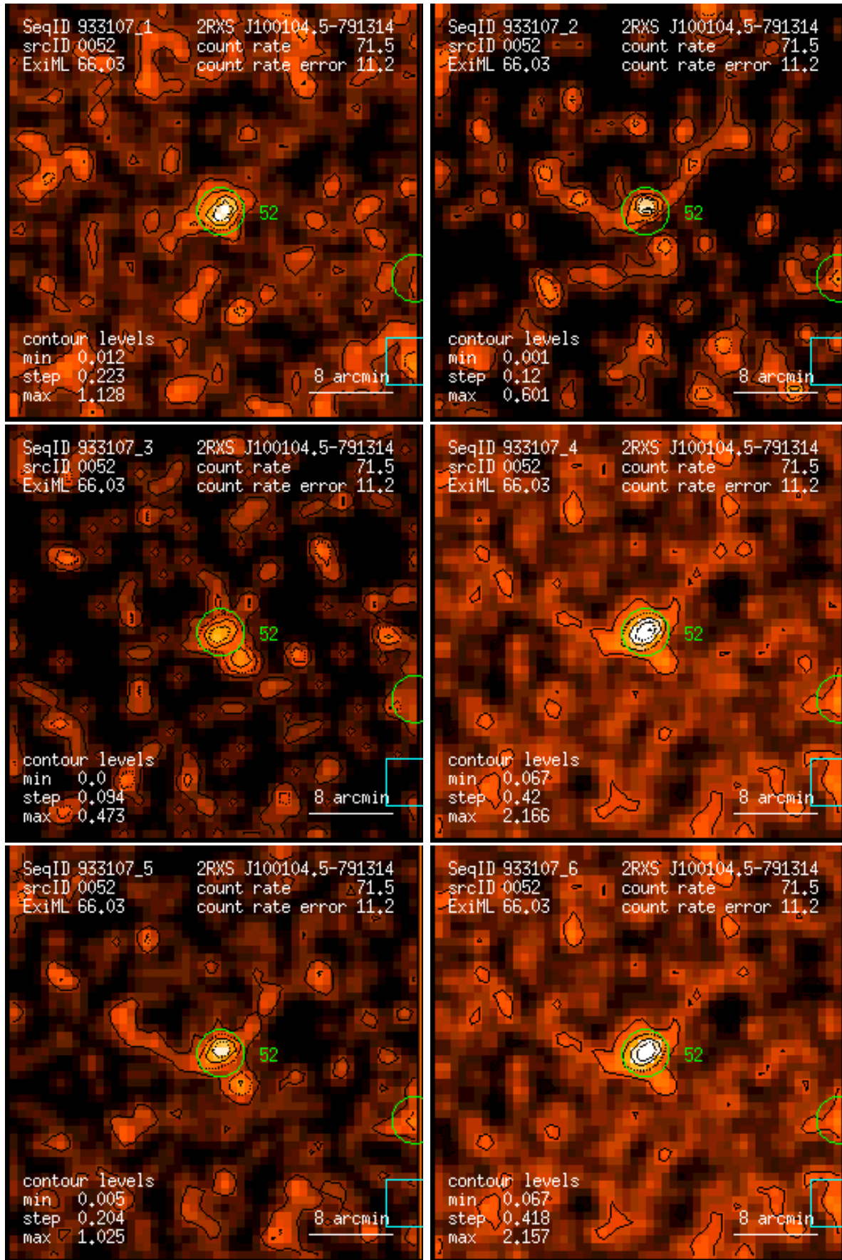
Figure 52: RASS 933107: detection 0052: band rate images, Gaussian filter: (1) PSPC channels 11 – 41, (2) 52 – 90, (3) 91 – 201, (4) 11 – 235, (5) 52 – 201, (6) 11 – 201. Broad band rates in counts/ks. Band rate contour levels in counts/ks/arcmin 2 .
