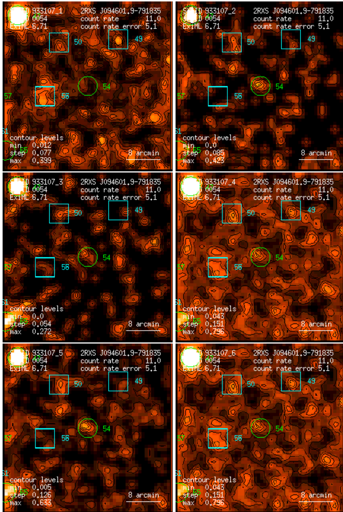
Figure 54: RASS 933107: detection 0054: band rate images, Gaussian filter: (1) PSPC channels 11 – 41, (2) 52 – 90, (3) 91 – 201, (4) 11 – 235, (5) 52 – 201, (6) 11 – 201. Broad band rates in counts/ks. Band rate contour levels in counts/ks/arcmin 2 .
