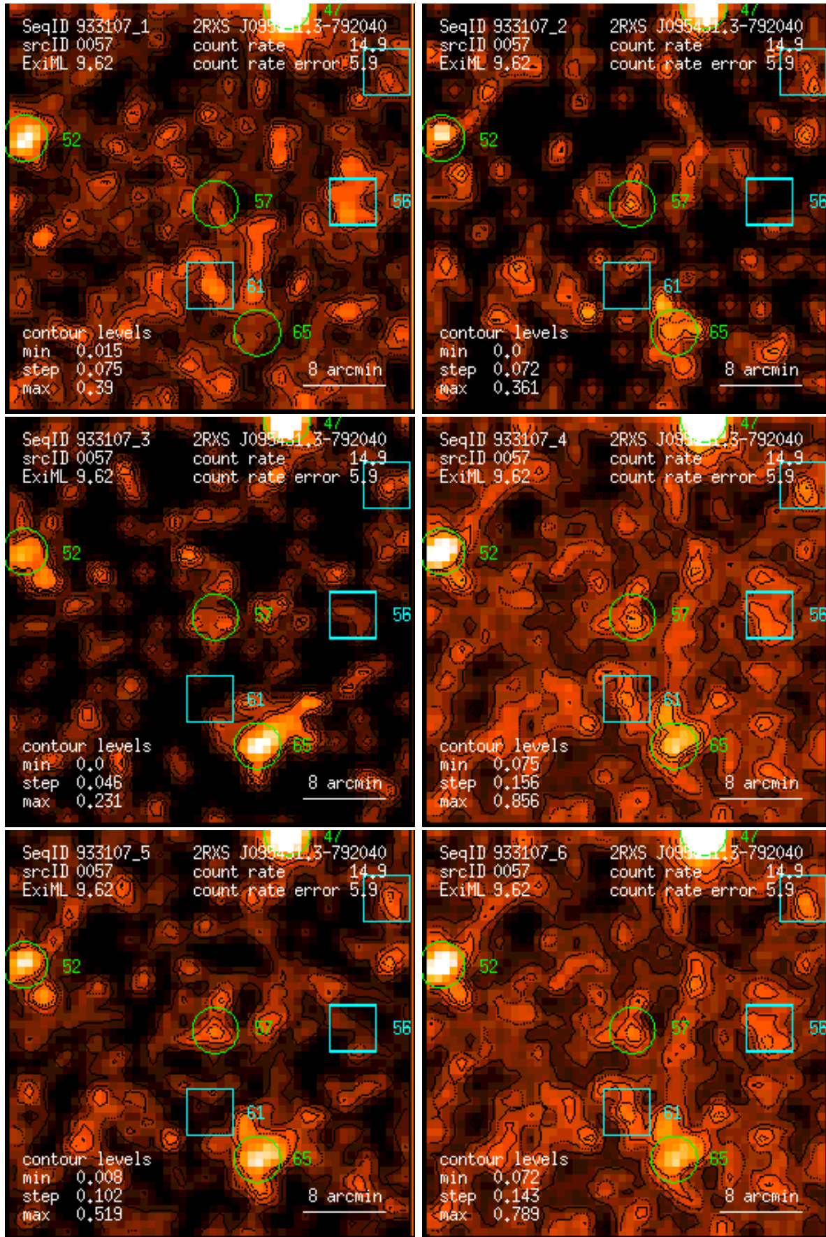
Figure 57: RASS 933107: detection 0057: band rate images, Gaussian filter: (1) PSPC channels 11 – 41, (2) 52 – 90, (3) 91 – 201, (4) 11 – 235, (5) 52 – 201, (6) 11 – 201. Broad band rates in counts/ks. Band rate contour levels in counts/ks/arcmin 2 .
