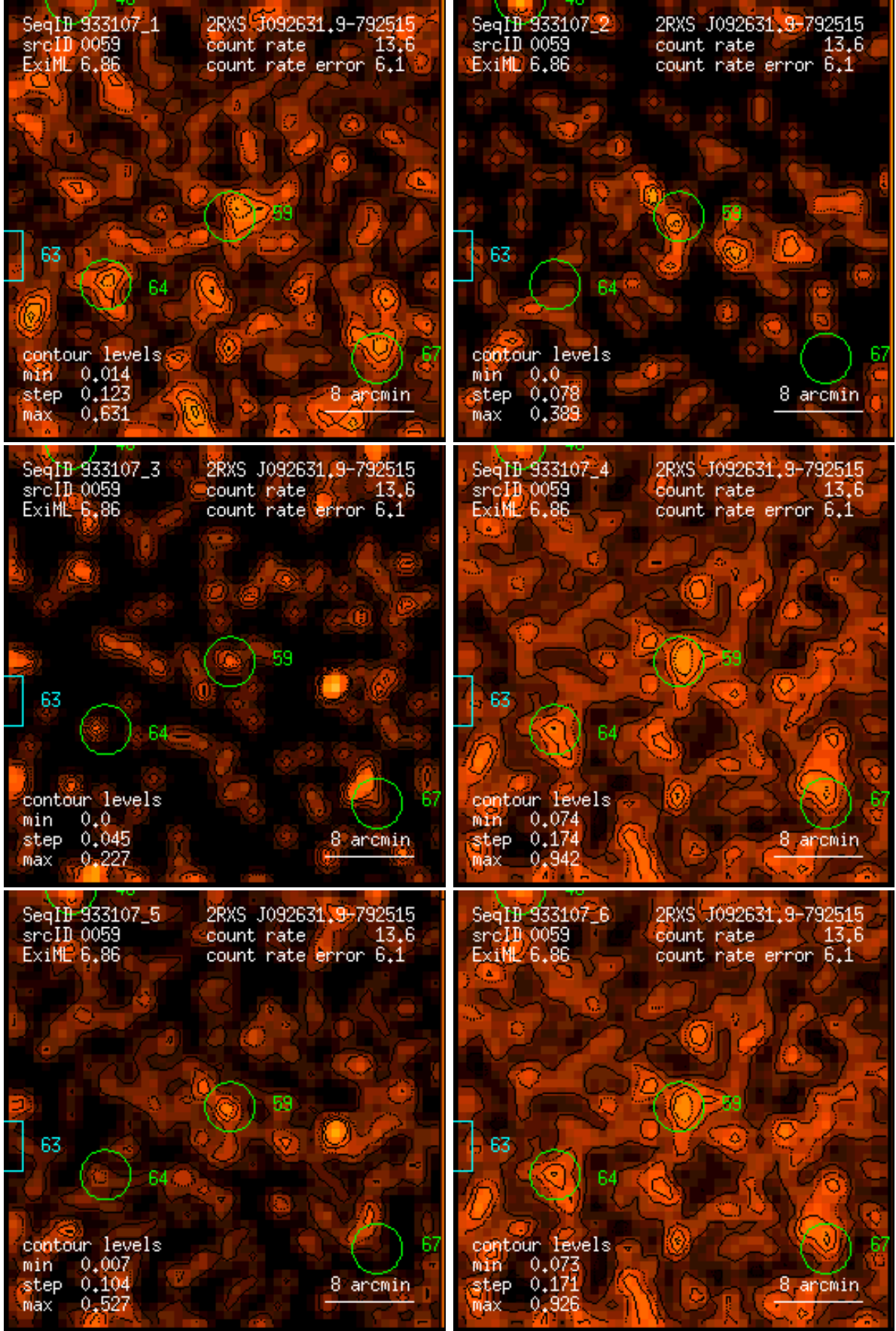
Figure 59: RASS 933107: detection 0059: band rate images, Gaussian filter: (1) PSPC channels 11 – 41, (2) 52 – 90, (3) 91 – 201, (4) 11 – 235, (5) 52 – 201, (6) 11 – 201. Broad band rates in counts/ks. Band rate contour levels in counts/ks/arcmin 2 .
