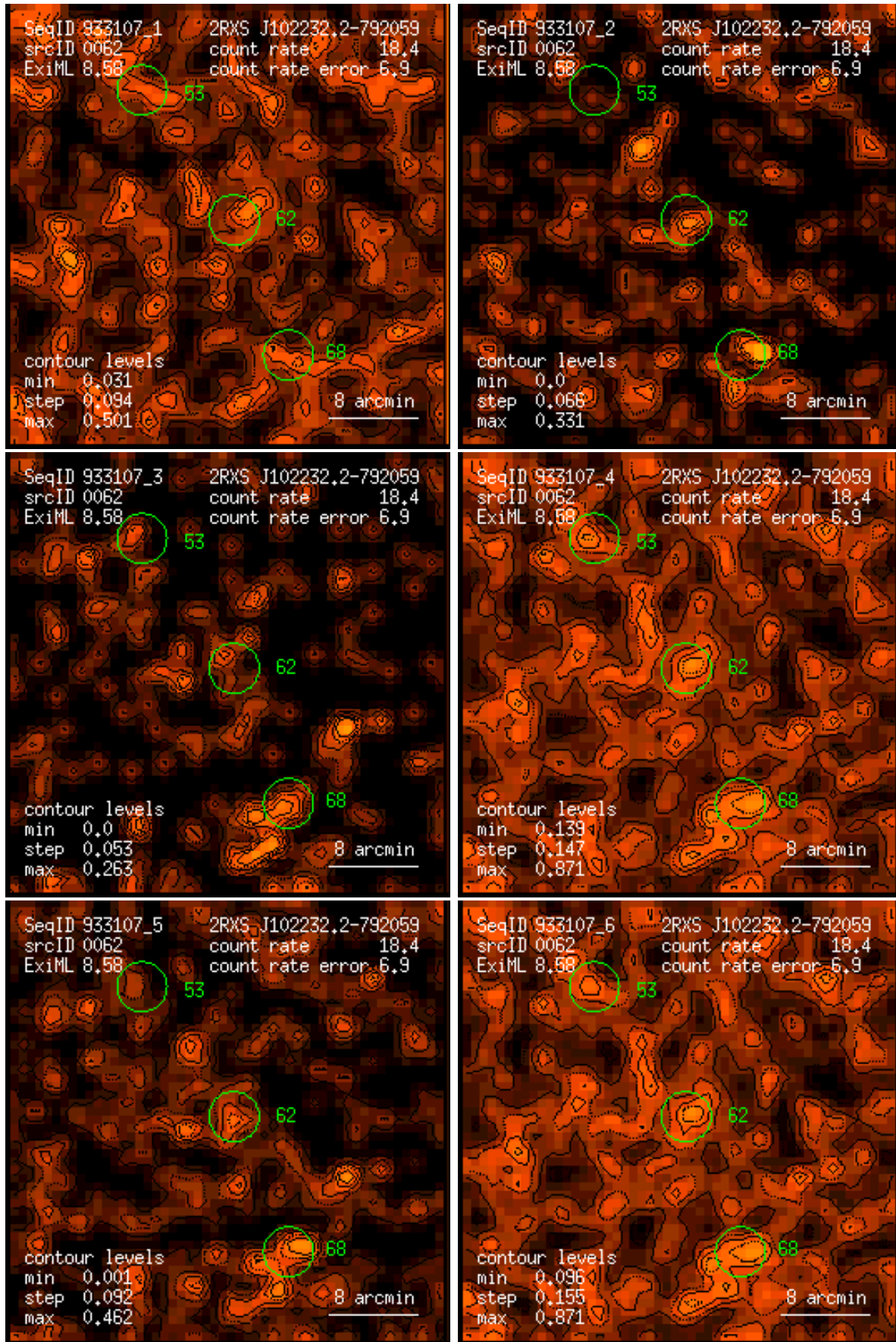
Figure 62: RASS 933107: detection 0062: band rate images, Gaussian filter: (1) PSPC channels 11 – 41, (2) 52 – 90, (3) 91 – 201, (4) 11 – 235, (5) 52 – 201, (6) 11 – 201. Broad band rates in counts/ks. Band rate contour levels in counts/ks/arcmin 2 .
