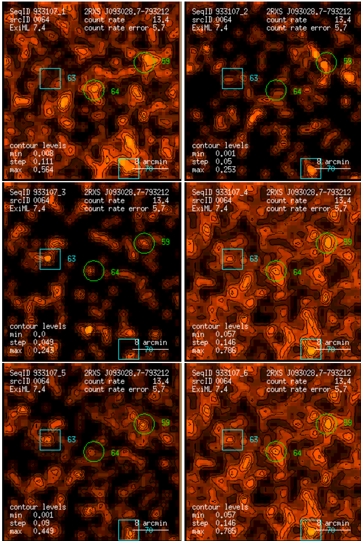
Figure 64: RASS 933107: detection 0064: band rate images, Gaussian filter: (1) PSPC channels 11 – 41, (2) 52 – 90, (3) 91 – 201, (4) 11 – 235, (5) 52 – 201, (6) 11 – 201. Broad band rates in counts/ks. Band rate contour levels in counts/ks/arcmin 2 .
