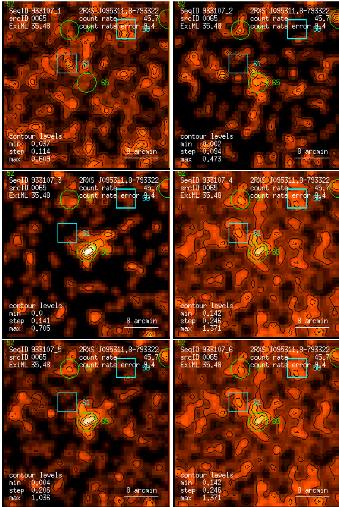
Figure 65: RASS 933107: detection 0065: band rate images, Gaussian filter: (1) PSPC channels 11 – 41, (2) 52 – 90, (3) 91 – 201, (4) 11 – 235, (5) 52 – 201, (6) 11 – 201. Broad band rates in counts/ks. Band rate contour levels in counts/ks/arcmin 2 .
