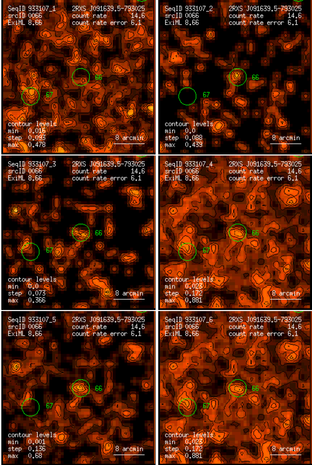
Figure 66: RASS 933107: detection 0066: band rate images, Gaussian filter: (1) PSPC channels 11 – 41, (2) 52 – 90, (3) 91 – 201, (4) 11 – 235, (5) 52 – 201, (6) 11 – 201. Broad band rates in counts/ks. Band rate contour levels in counts/ks/arcmin 2 .
