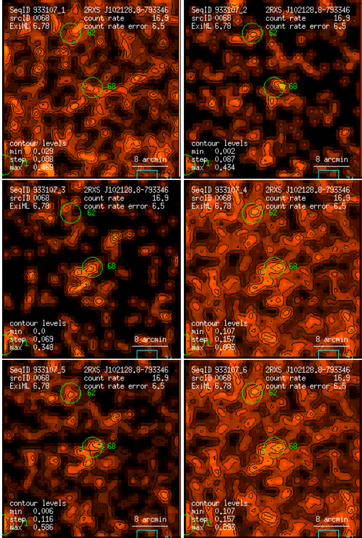
Figure 68: RASS 933107: detection 0068: band rate images, Gaussian filter: (1) PSPC channels 11 – 41, (2) 52 – 90, (3) 91 – 201, (4) 11 – 235, (5) 52 – 201, (6) 11 – 201. Broad band rates in counts/ks. Band rate contour levels in counts/ks/arcmin 2 .
