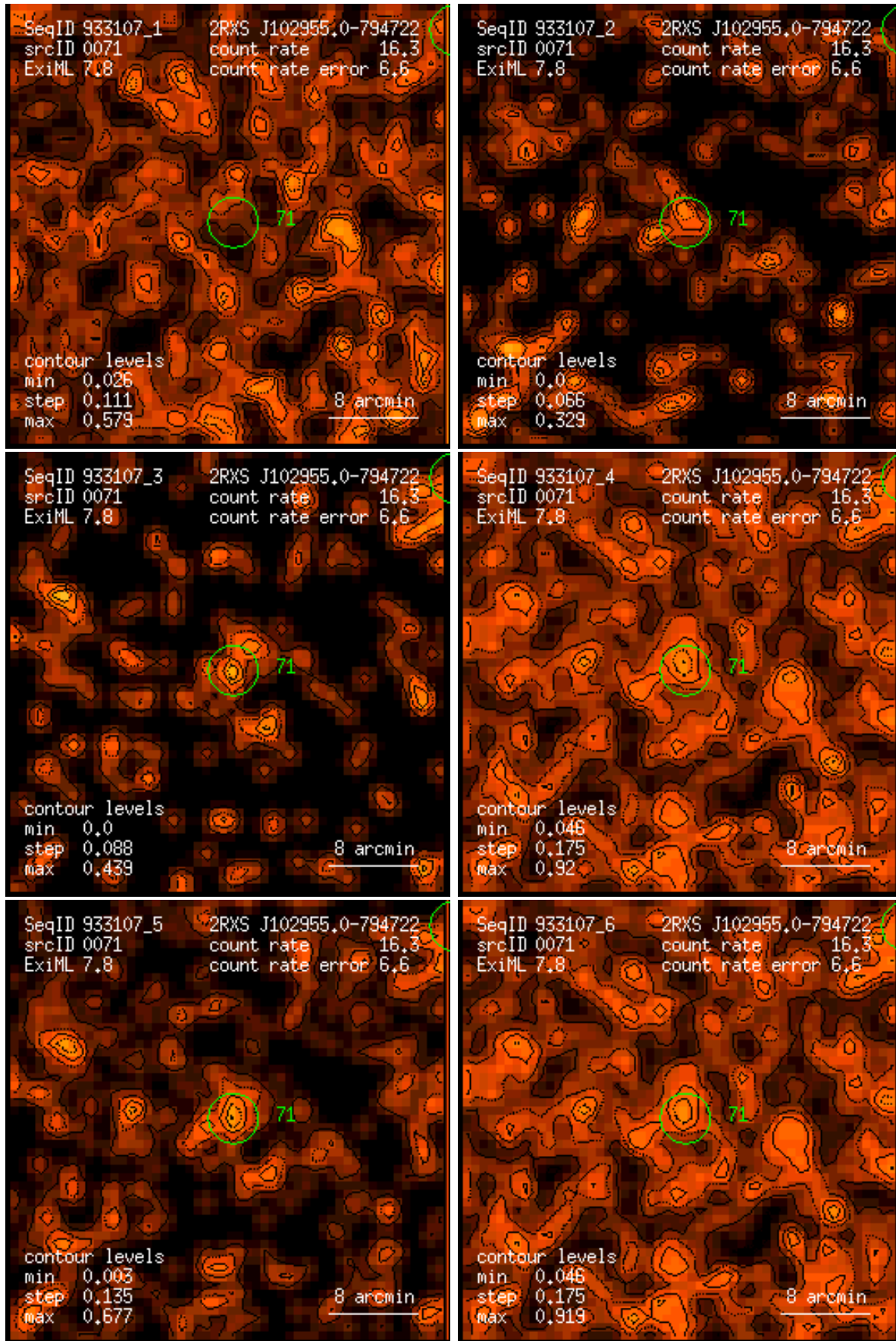
Figure 71: RASS 933107: detection 0071: band rate images, Gaussian filter: (1) PSPC channels 11 – 41, (2) 52 – 90, (3) 91 – 201, (4) 11 – 235, (5) 52 – 201, (6) 11 – 201. Broad band rates in counts/ks. Band rate contour levels in counts/ks/arcmin 2 .
