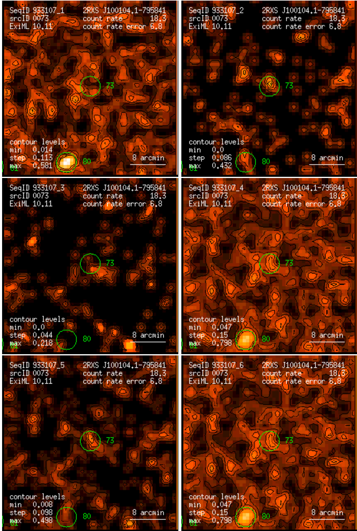
Figure 73: RASS 933107: detection 0073: band rate images, Gaussian filter: (1) PSPC channels 11 – 41, (2) 52 – 90, (3) 91 – 201, (4) 11 – 235, (5) 52 – 201, (6) 11 – 201. Broad band rates in counts/ks. Band rate contour levels in counts/ks/arcmin 2 .
