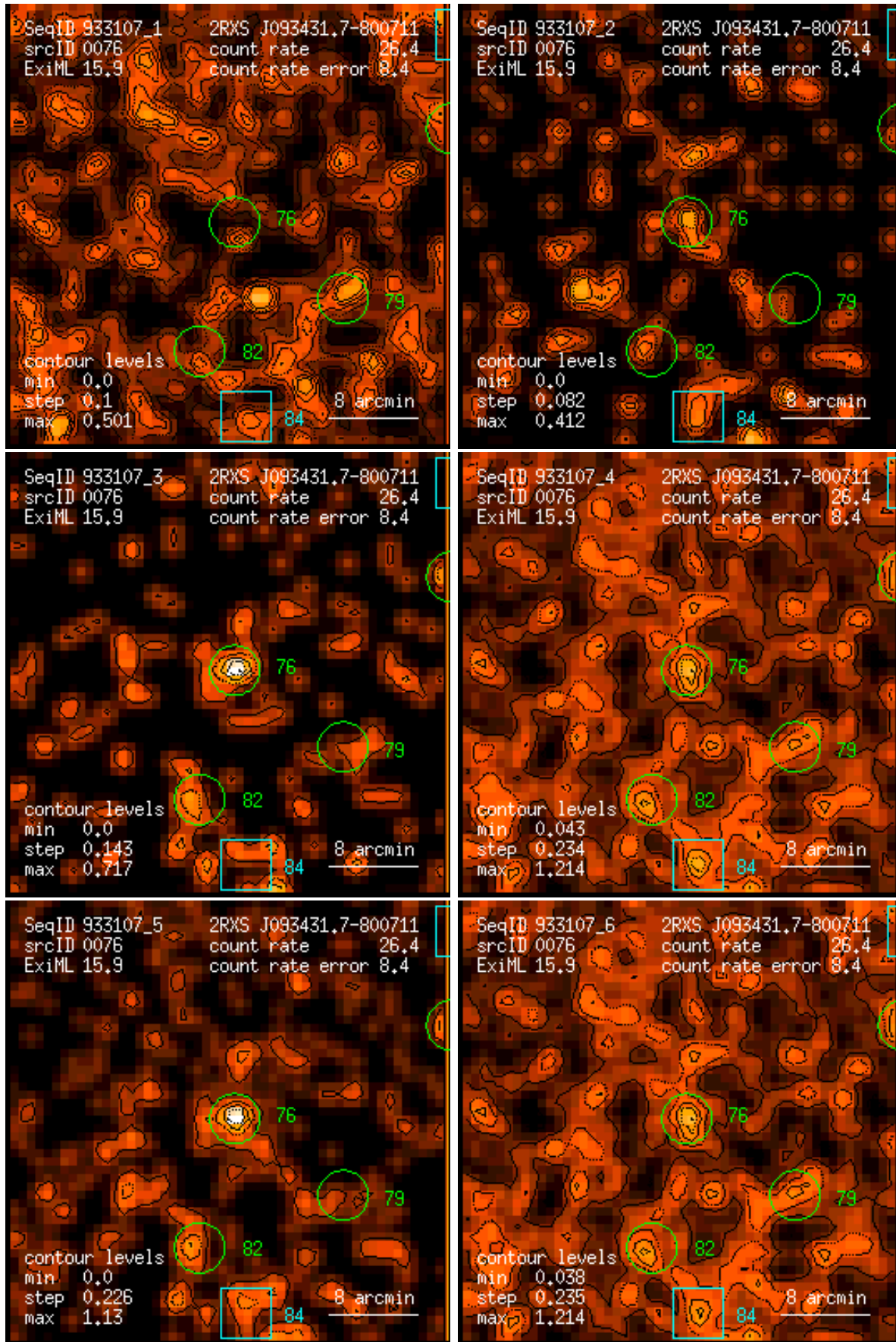
Figure 76: RASS 933107: detection 0076: band rate images, Gaussian filter: (1) PSPC channels 11 – 41, (2) 52 – 90, (3) 91 – 201, (4) 11 – 235, (5) 52 – 201, (6) 11 – 201. Broad band rates in counts/ks. Band rate contour levels in counts/ks/arcmin 2 .
