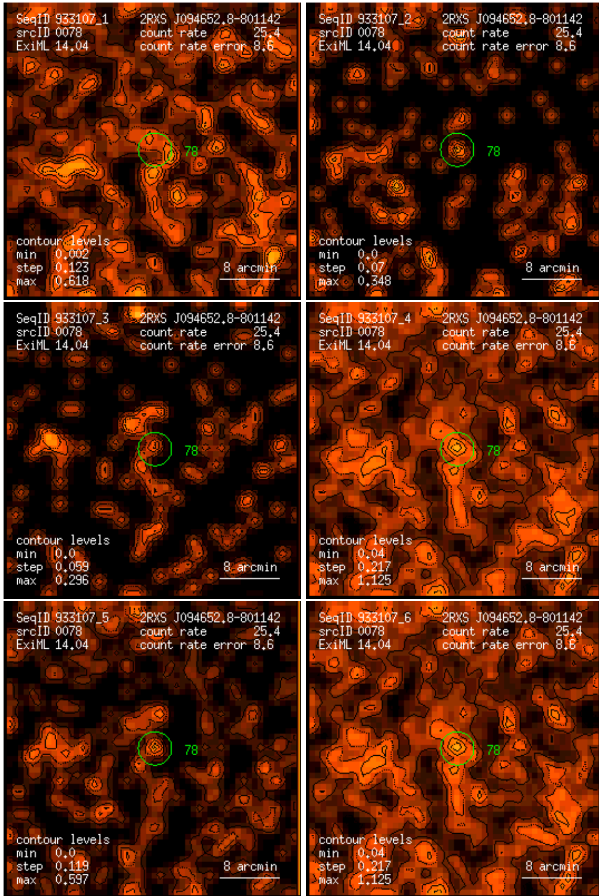
Figure 78: RASS 933107: detection 0078: band rate images, Gaussian filter: (1) PSPC channels 11 – 41, (2) 52 – 90, (3) 91 – 201, (4) 11 – 235, (5) 52 – 201, (6) 11 – 201. Broad band rates in counts/ks. Band rate contour levels in counts/ks/arcmin 2 .
