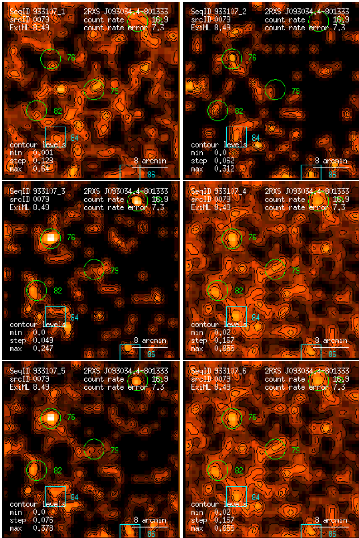
Figure 79: RASS 933107: detection 0079: band rate images, Gaussian filter: (1) PSPC channels 11 – 41, (2) 52 – 90, (3) 91 – 201, (4) 11 – 235, (5) 52 – 201, (6) 11 – 201. Broad band rates in counts/ks. Band rate contour levels in counts/ks/arcmin 2 .
