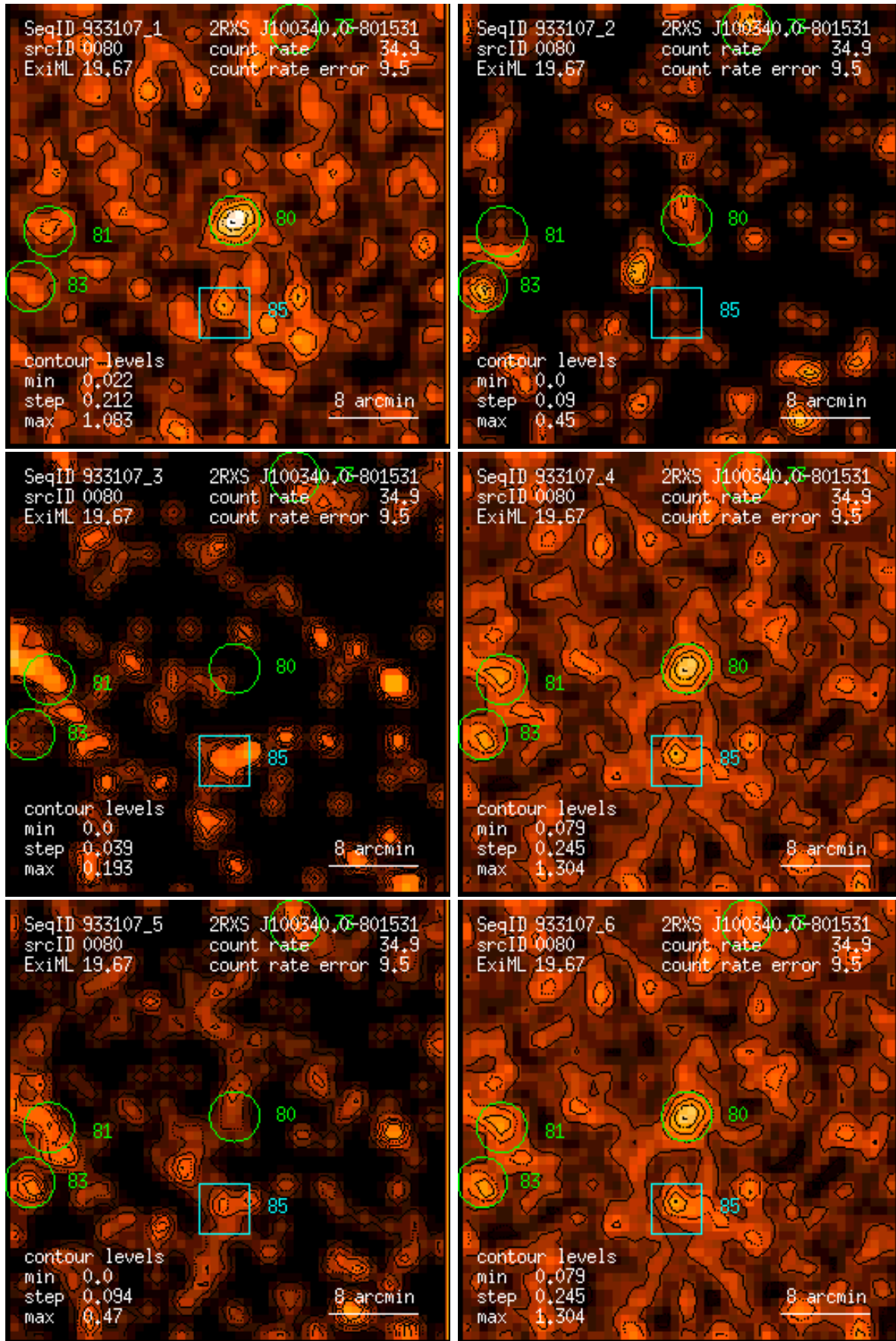
Figure 80: RASS 933107: detection 0080: band rate images, Gaussian filter: (1) PSPC channels 11 – 41, (2) 52 – 90, (3) 91 – 201, (4) 11 – 235, (5) 52 – 201, (6) 11 – 201. Broad band rates in counts/ks. Band rate contour levels in counts/ks/arcmin 2 .
