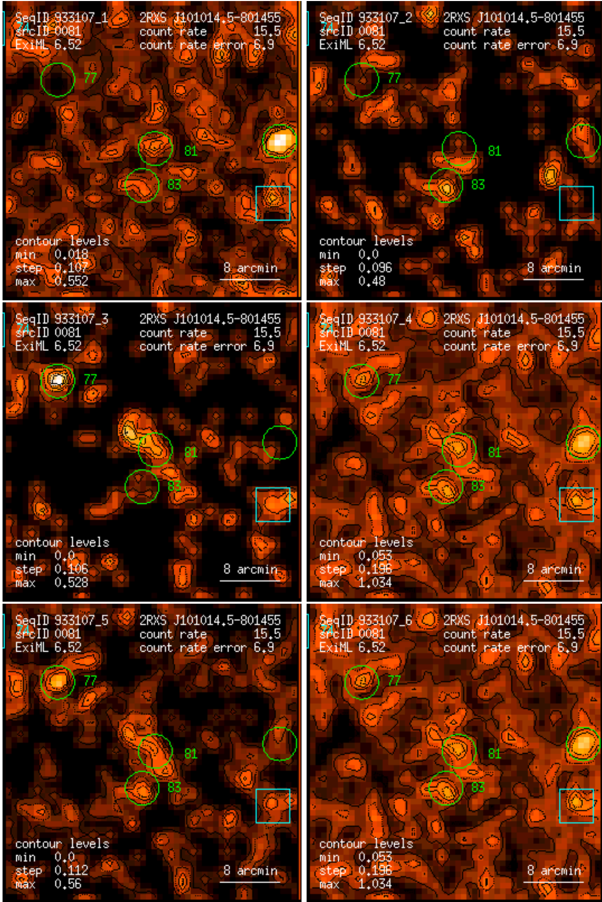
Figure 81: RASS 933107: detection 0081: band rate images, Gaussian filter: (1) PSPC channels 11 – 41, (2) 52 – 90, (3) 91 – 201, (4) 11 – 235, (5) 52 – 201, (6) 11 – 201. Broad band rates in counts/ks. Band rate contour levels in counts/ks/arcmin 2 .
