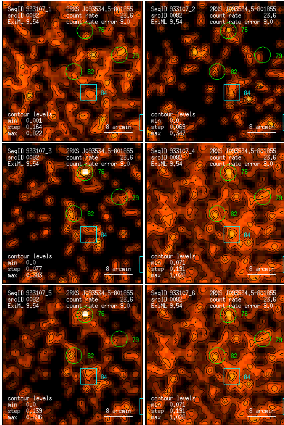
Figure 82: RASS 933107: detection 0082: band rate images, Gaussian filter: (1) PSPC channels 11 – 41, (2) 52 – 90, (3) 91 – 201, (4) 11 – 235, (5) 52 – 201, (6) 11 – 201. Broad band rates in counts/ks. Band rate contour levels in counts/ks/arcmin 2 .
