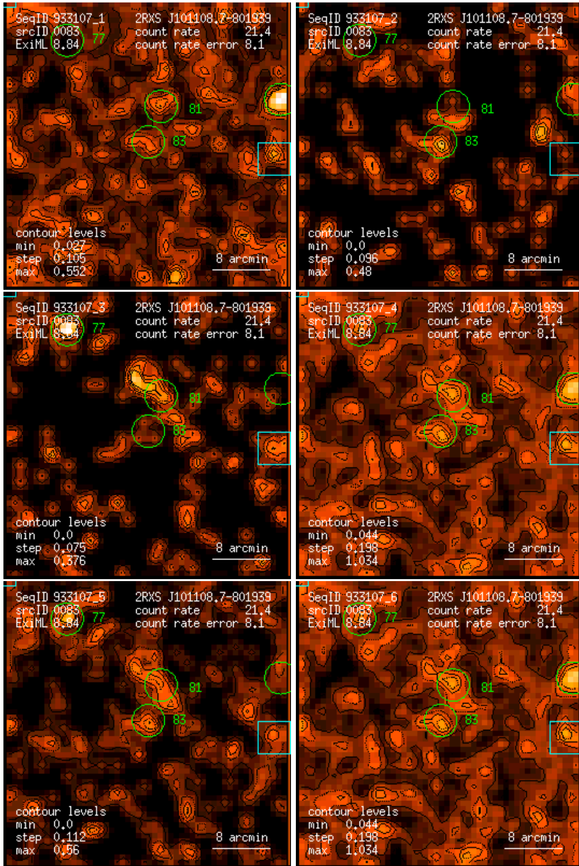
Figure 83: RASS 933107: detection 0083: band rate images, Gaussian filter: (1) PSPC channels 11 – 41, (2) 52 – 90, (3) 91 – 201, (4) 11 – 235, (5) 52 – 201, (6) 11 – 201. Broad band rates in counts/ks. Band rate contour levels in counts/ks/arcmin 2 .
