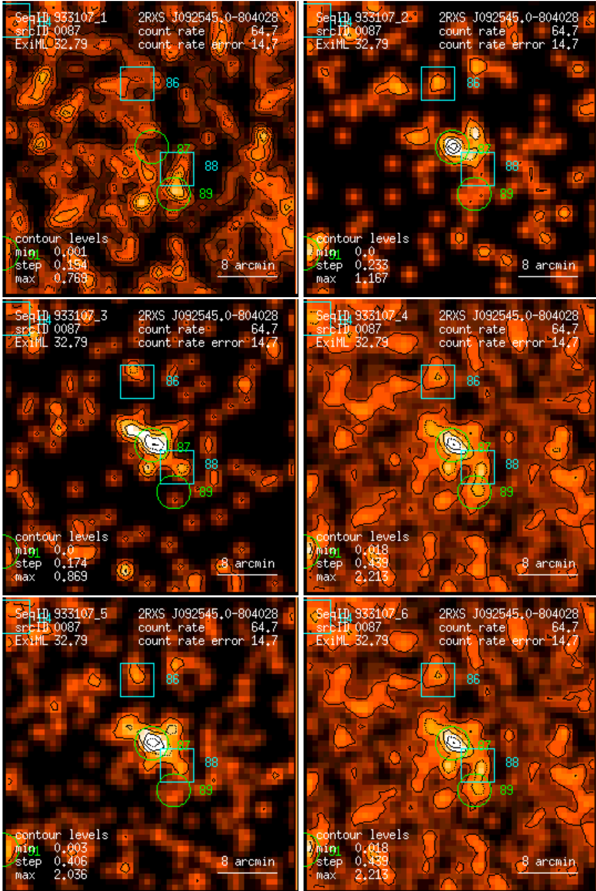
Figure 87: RASS 933107: detection 0087: band rate images, Gaussian filter: (1) PSPC channels 11 – 41, (2) 52 – 90, (3) 91 – 201, (4) 11 – 235, (5) 52 – 201, (6) 11 – 201. Broad band rates in counts/ks. Band rate contour levels in counts/ks/arcmin 2 .
