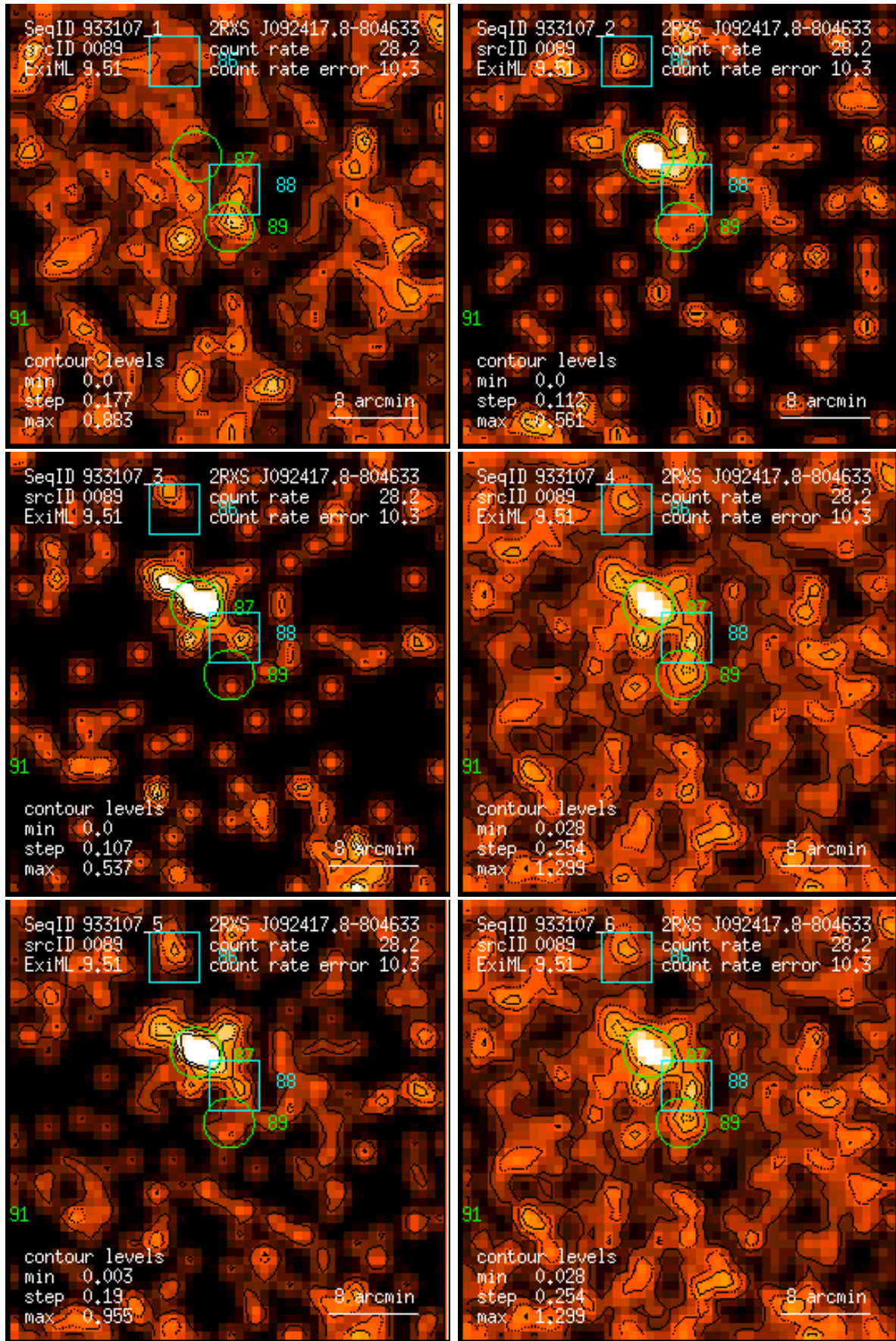
Figure 89: RASS 933107: detection 0089: band rate images, Gaussian filter: (1) PSPC channels 11 – 41, (2) 52 – 90, (3) 91 – 201, (4) 11 – 235, (5) 52 – 201, (6) 11 – 201. Broad band rates in counts/ks. Band rate contour levels in counts/ks/arcmin 2 .
