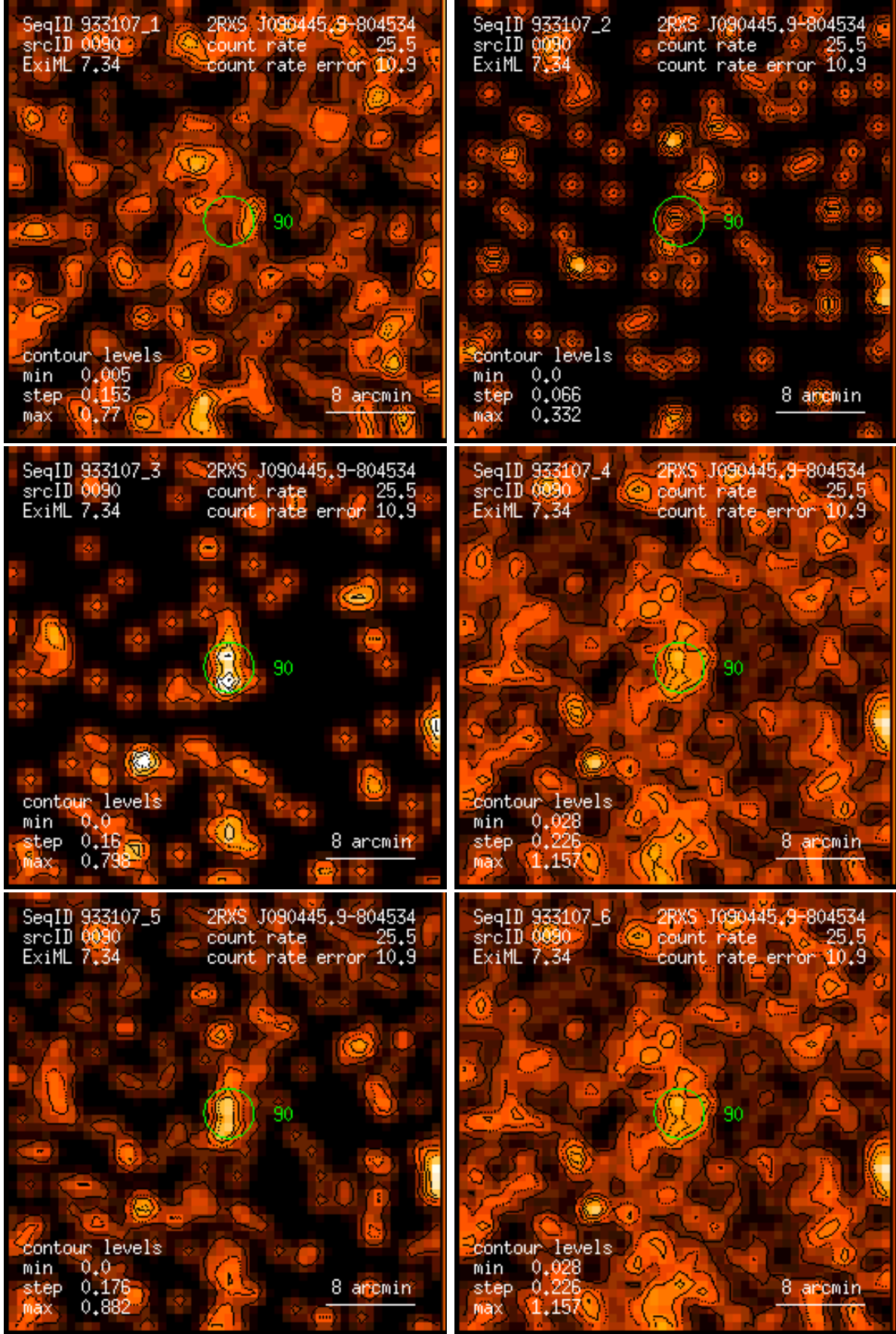
Figure 90: RASS 933107: detection 0090: band rate images, Gaussian filter: (1) PSPC channels 11 – 41, (2) 52 – 90, (3) 91 – 201, (4) 11 – 235, (5) 52 – 201, (6) 11 – 201. Broad band rates in counts/ks. Band rate contour levels in counts/ks/arcmin 2 .
