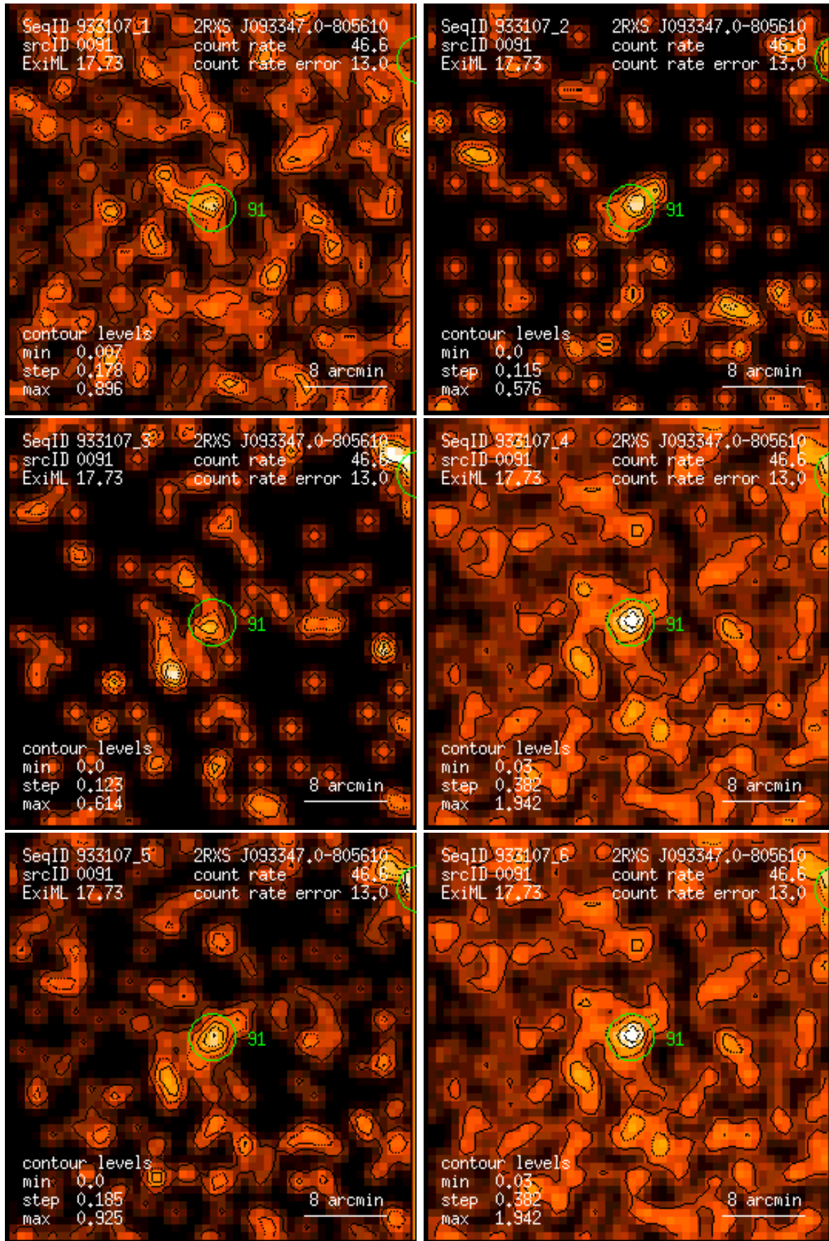
Figure 91: RASS 933107: detection 0091: band rate images, Gaussian filter: (1) PSPC channels 11 – 41, (2) 52 – 90, (3) 91 – 201, (4) 11 – 235, (5) 52 – 201, (6) 11 – 201. Broad band rates in counts/ks. Band rate contour levels in counts/ks/arcmin 2 .
