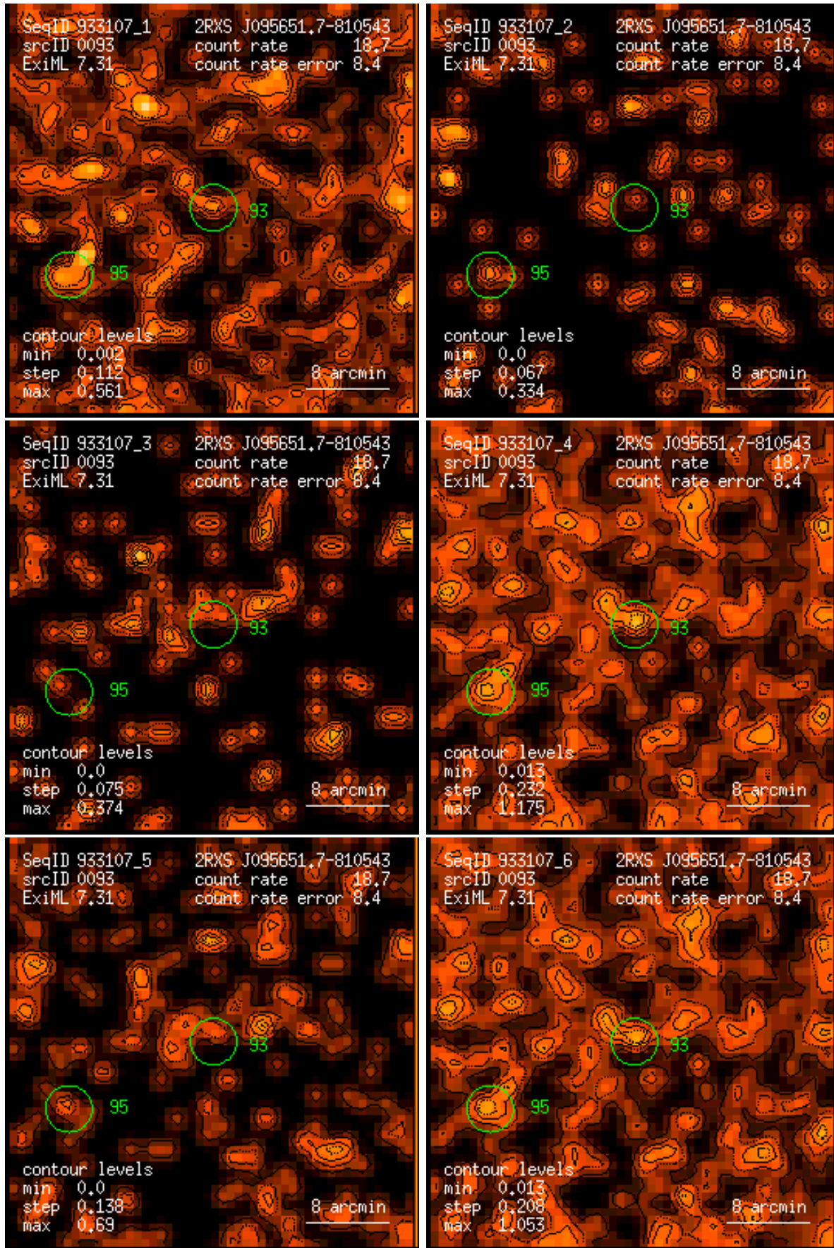
Figure 93: RASS 933107: detection 0093: band rate images, Gaussian filter: (1) PSPC channels 11 – 41, (2) 52 – 90, (3) 91 – 201, (4) 11 – 235, (5) 52 – 201, (6) 11 – 201. Broad band rates in counts/ks. Band rate contour levels in counts/ks/arcmin 2 .
