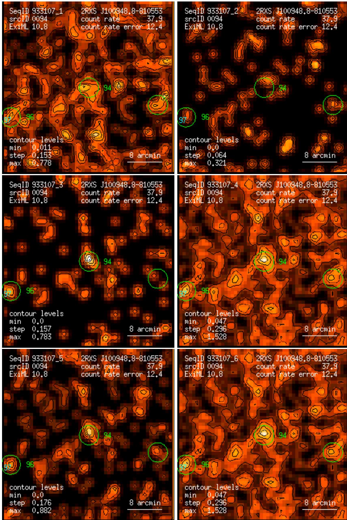
Figure 94: RASS 933107: detection 0094: band rate images, Gaussian filter: (1) PSPC channels 11 – 41, (2) 52 – 90, (3) 91 – 201, (4) 11 – 235, (5) 52 – 201, (6) 11 – 201. Broad band rates in counts/ks. Band rate contour levels in counts/ks/arcmin 2 .
