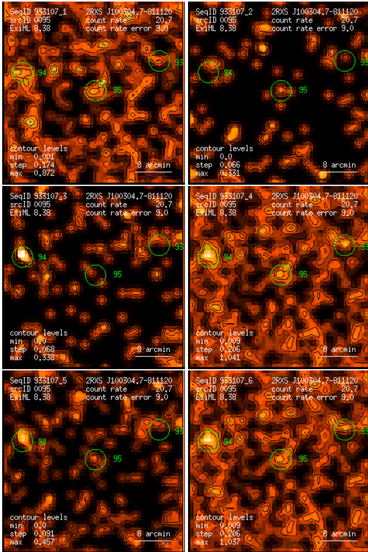
Figure 95: RASS 933107: detection 0095: band rate images, Gaussian filter: (1) PSPC channels 11 – 41, (2) 52 – 90, (3) 91 – 201, (4) 11 – 235, (5) 52 – 201, (6) 11 – 201. Broad band rates in counts/ks. Band rate contour levels in counts/ks/arcmin 2 .
