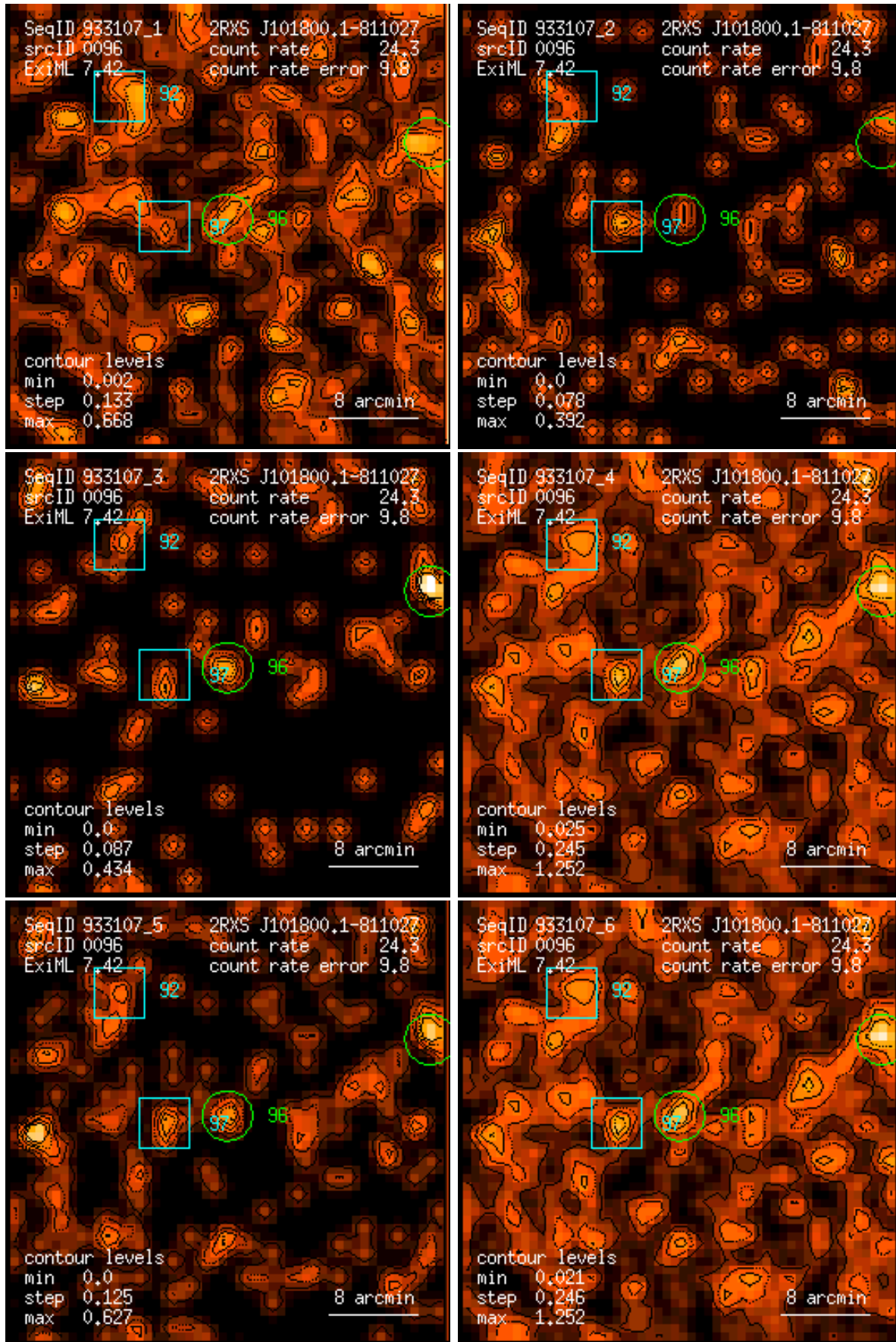
Figure 96: RASS 933107: detection 0096: band rate images, Gaussian filter: (1) PSPC channels 11 – 41, (2) 52 – 90, (3) 91 – 201, (4) 11 – 235, (5) 52 – 201, (6) 11 – 201. Broad band rates in counts/ks. Band rate contour levels in counts/ks/arcmin 2 .
