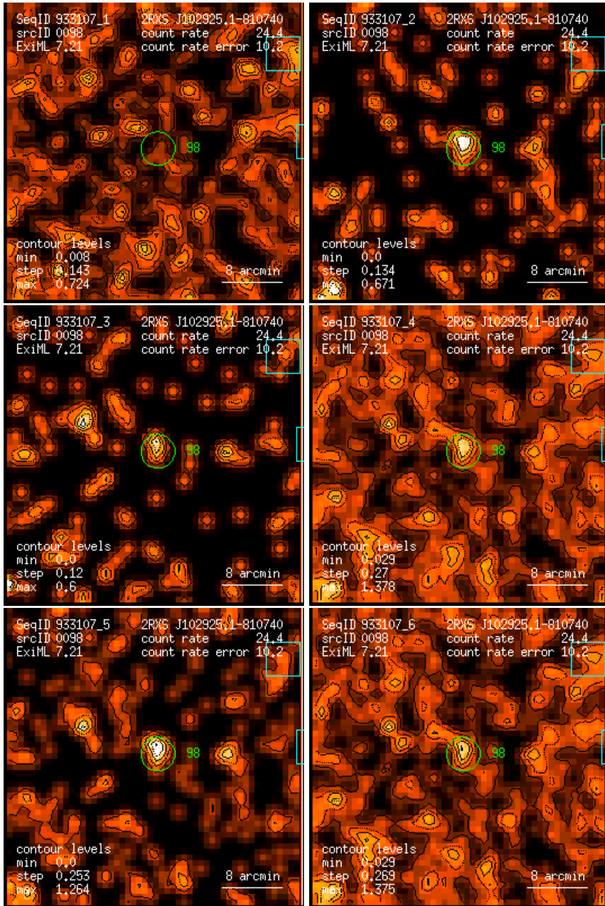
Figure 98: RASS 933107: detection 0098: band rate images, Gaussian filter: (1) PSPC channels 11 – 41, (2) 52 – 90, (3) 91 – 201, (4) 11 – 235, (5) 52 – 201, (6) 11 – 201. Broad band rates in counts/ks. Band rate contour levels in counts/ks/arcmin 2 .
