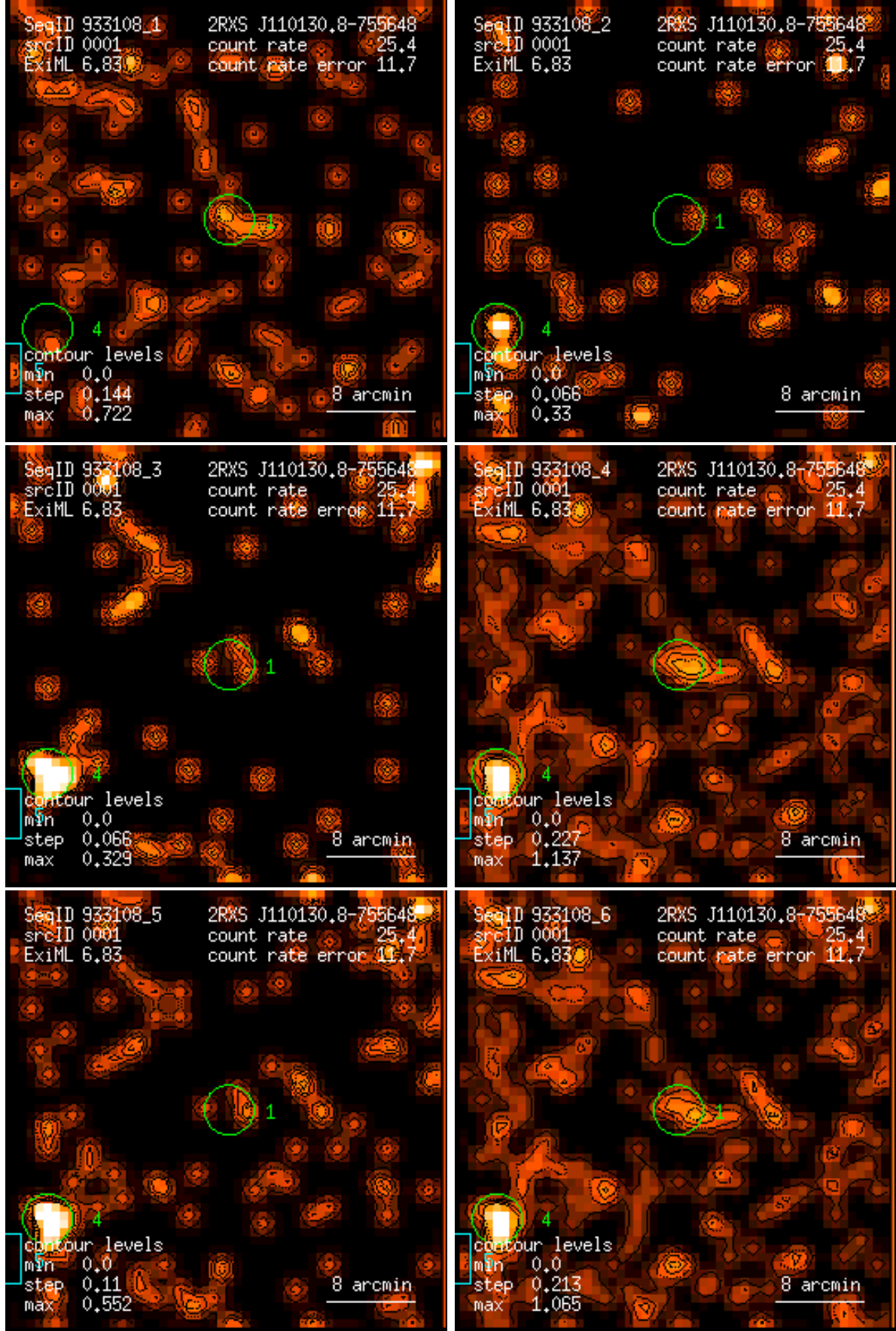
Figure 1: RASS 933108: detection 0001: band rate images, Gaussian filter: (1) PSPC channels 11 – 41, (2) 52 – 90, (3) 91 – 201, (4) 11 – 235, (5) 52 – 201, (6) 11 – 201. Broad band rates in counts/ks. Band rate contour levels in counts/ks/arcmin 2 .
