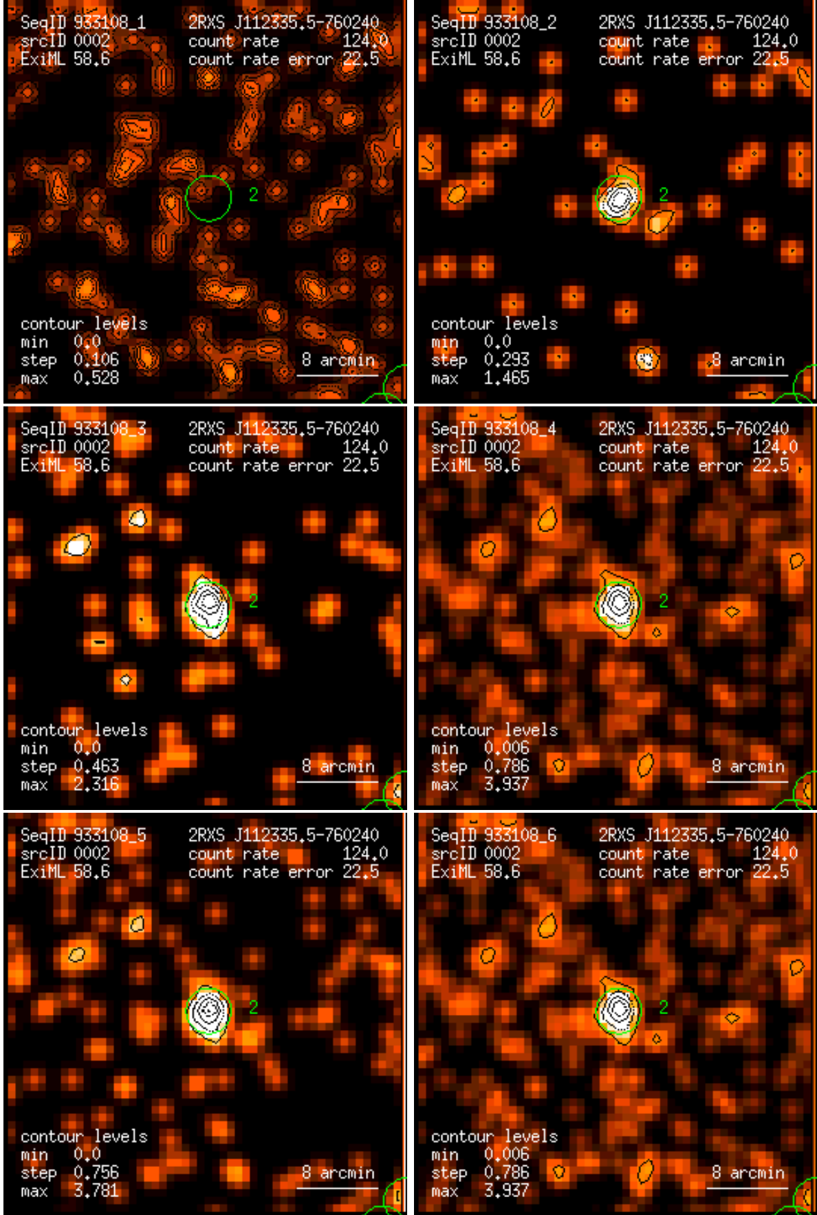
Figure 2: RASS 933108: detection 0002: band rate images, Gaussian filter: (1) PSPC channels 11 – 41, (2) 52 – 90, (3) 91 – 201, (4) 11 – 235, (5) 52 – 201, (6) 11 – 201. Broad band rates in counts/ks. Band rate contour levels in counts/ks/arcmin 2 .
