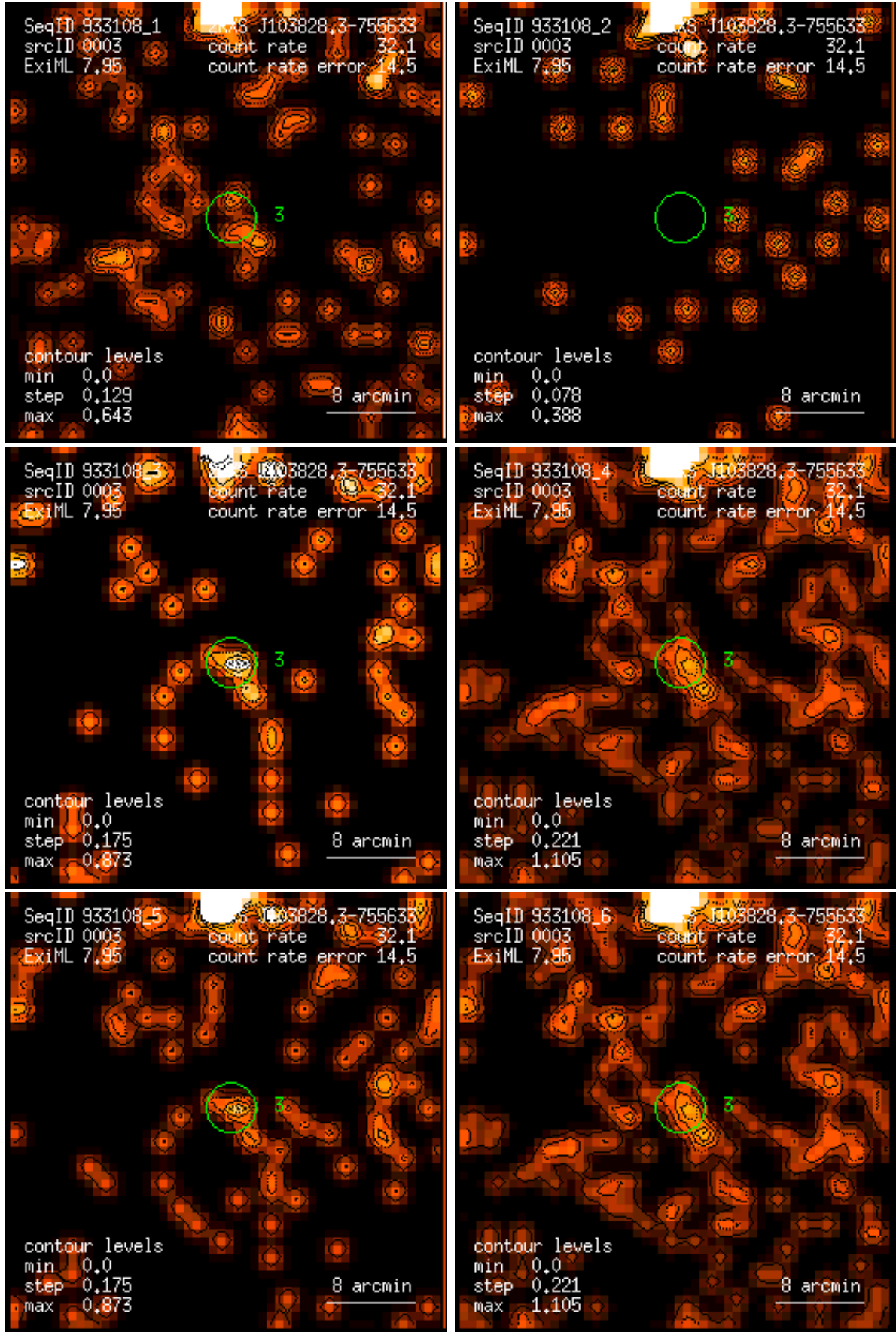
Figure 3: RASS 933108: detection 0003: band rate images, Gaussian filter: (1) PSPC channels 11 – 41, (2) 52 – 90, (3) 91 – 201, (4) 11 – 235, (5) 52 – 201, (6) 11 – 201. Broad band rates in counts/ks. Band rate contour levels in counts/ks/arcmin 2 .
