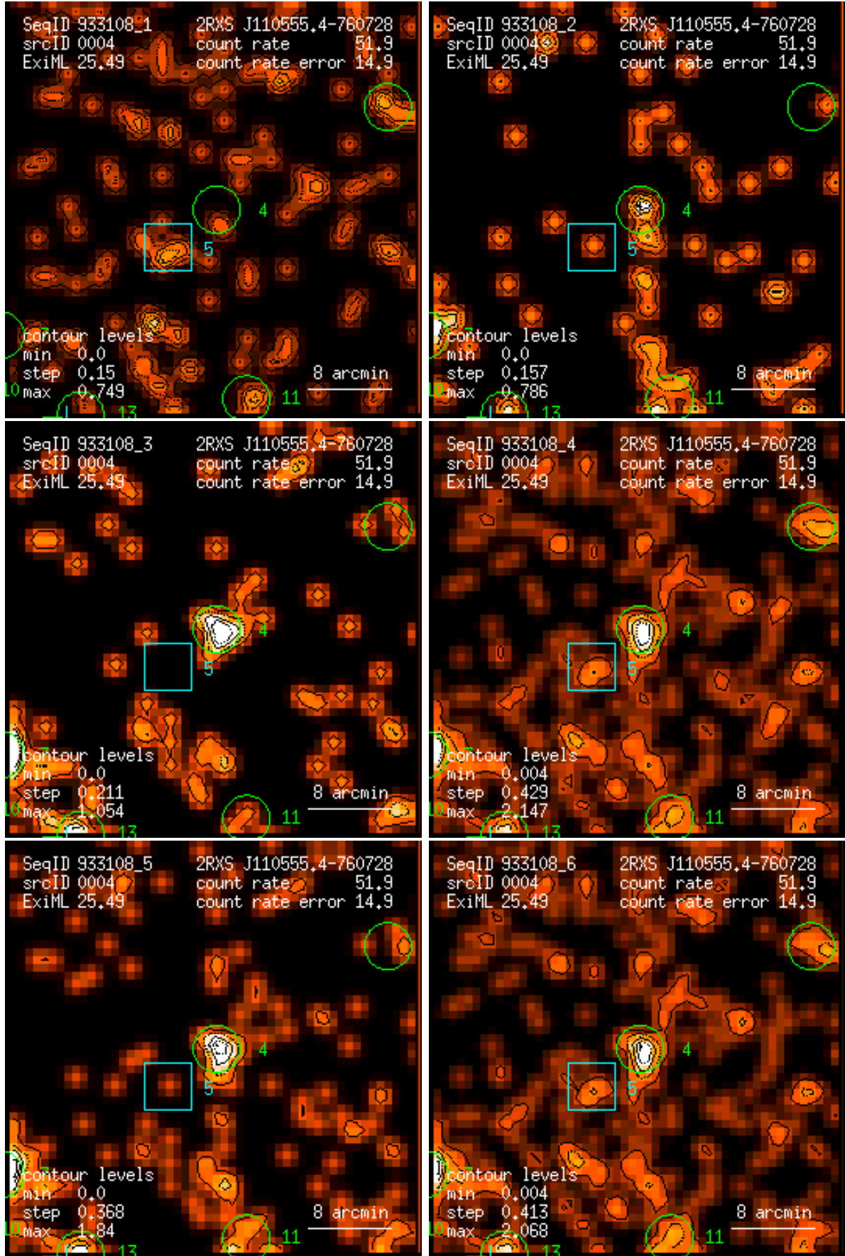
Figure 4: RASS 933108: detection 0004: band rate images, Gaussian filter: (1) PSPC channels 11 – 41, (2) 52 – 90, (3) 91 – 201, (4) 11 – 235, (5) 52 – 201, (6) 11 – 201. Broad band rates in counts/ks. Band rate contour levels in counts/ks/arcmin 2 .
