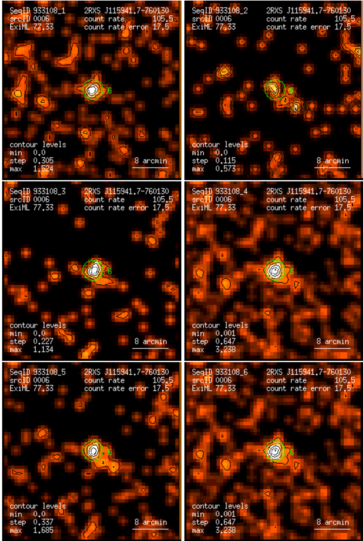
Figure 6: RASS 933108: detection 0006: band rate images, Gaussian filter: (1) PSPC channels 11 – 41, (2) 52 – 90, (3) 91 – 201, (4) 11 – 235, (5) 52 – 201, (6) 11 – 201. Broad band rates in counts/ks. Band rate contour levels in counts/ks/arcmin 2 .
