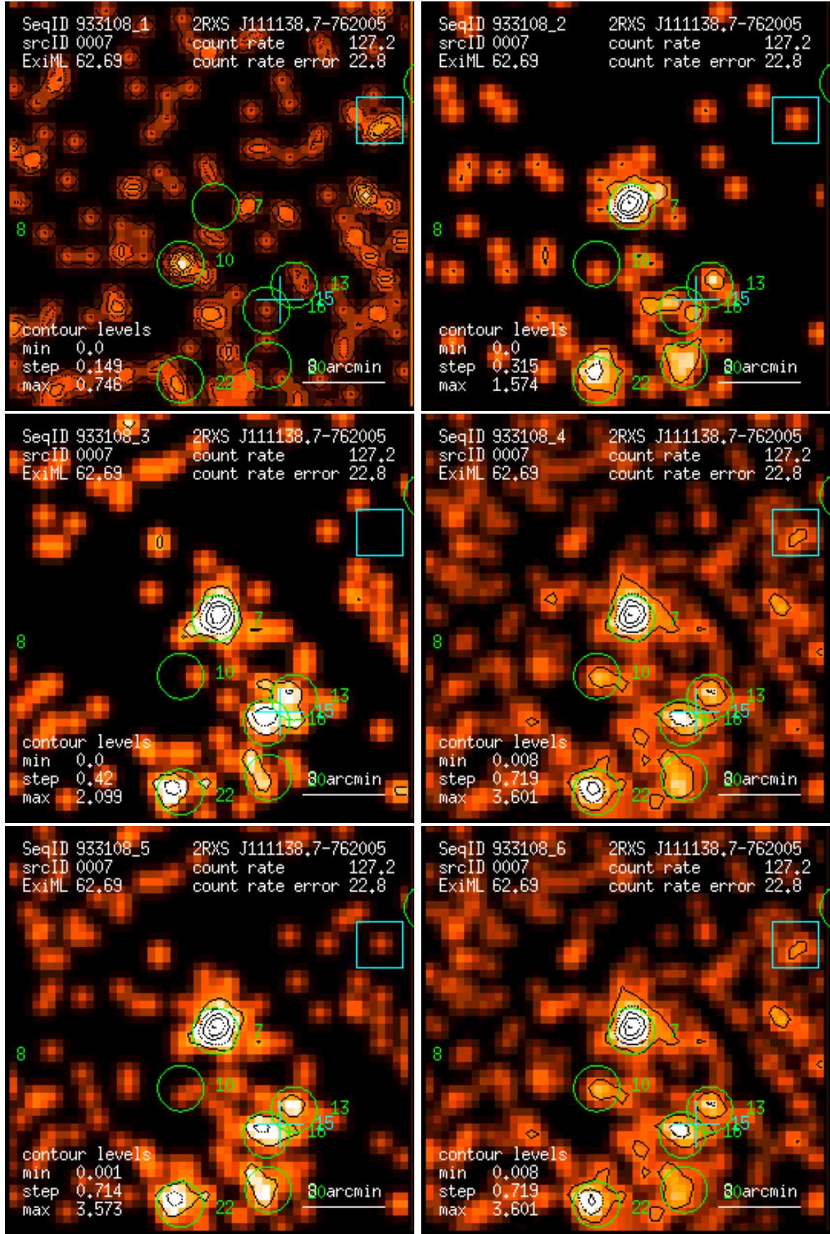
Figure 7: RASS 933108: detection 0007: band rate images, Gaussian filter: (1) PSPC channels 11 – 41, (2) 52 – 90, (3) 91 – 201, (4) 11 – 235, (5) 52 – 201, (6) 11 – 201. Broad band rates in counts/ks. Band rate contour levels in counts/ks/arcmin 2 .
