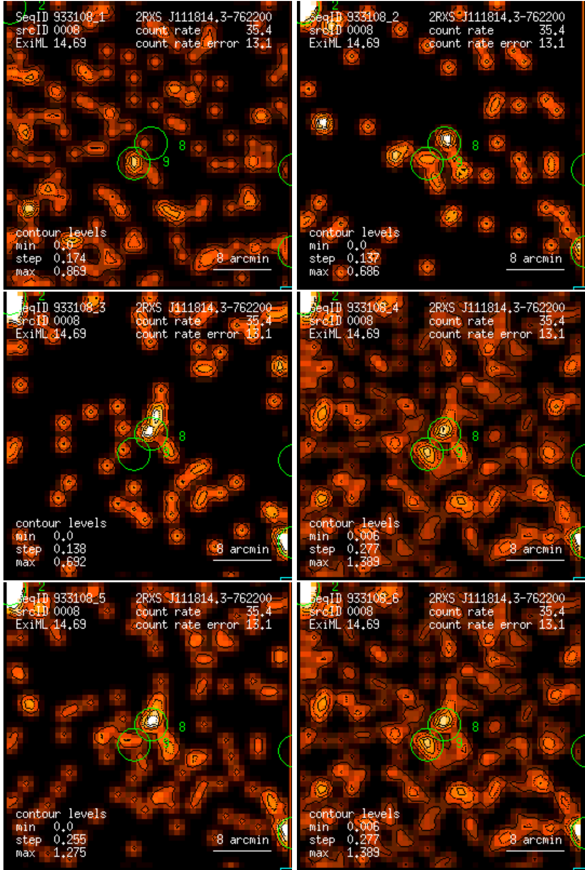
Figure 8: RASS 933108: detection 0008: band rate images, Gaussian filter: (1) PSPC channels 11 – 41, (2) 52 – 90, (3) 91 – 201, (4) 11 – 235, (5) 52 – 201, (6) 11 – 201. Broad band rates in counts/ks. Band rate contour levels in counts/ks/arcmin 2 .
