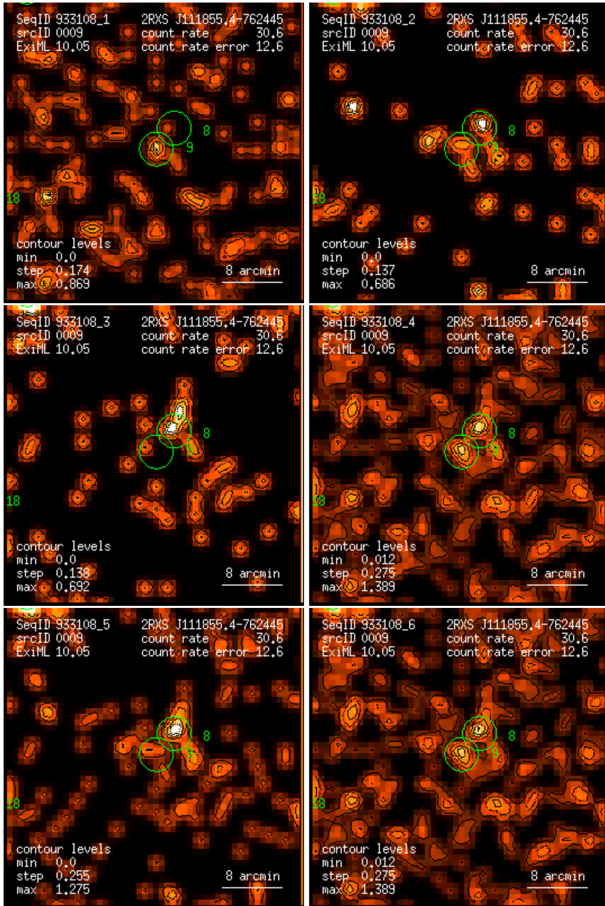
Figure 9: RASS 933108: detection 0009: band rate images, Gaussian filter: (1) PSPC channels 11 – 41, (2) 52 – 90, (3) 91 – 201, (4) 11 – 235, (5) 52 – 201, (6) 11 – 201. Broad band rates in counts/ks. Band rate contour levels in counts/ks/arcmin 2 .
