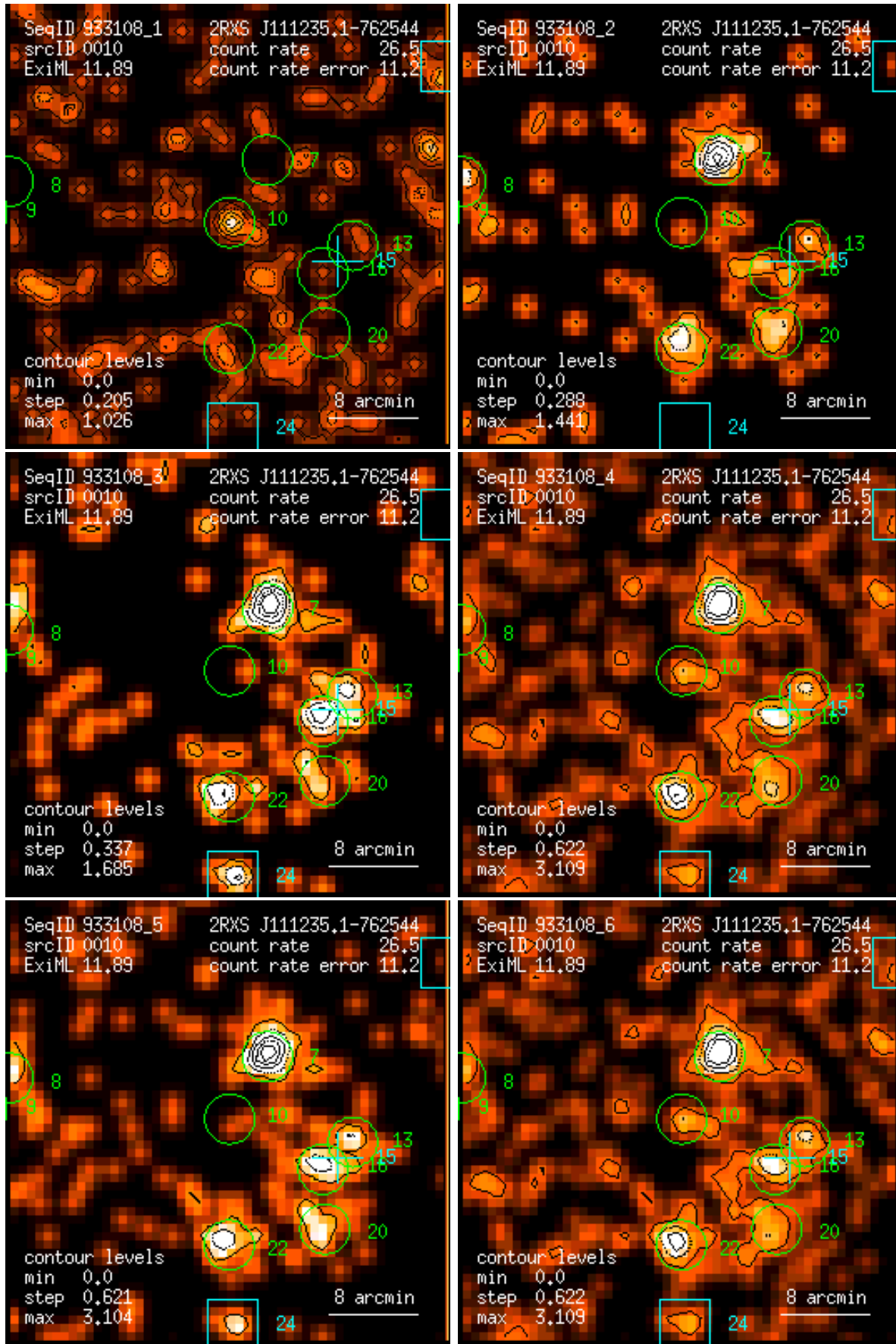
Figure 10: RASS 933108: detection 0010: band rate images, Gaussian filter: (1) PSPC channels 11 – 41, (2) 52 – 90, (3) 91 – 201, (4) 11 – 235, (5) 52 – 201, (6) 11 – 201. Broad band rates in counts/ks. Band rate contour levels in counts/ks/arcmin 2 .
