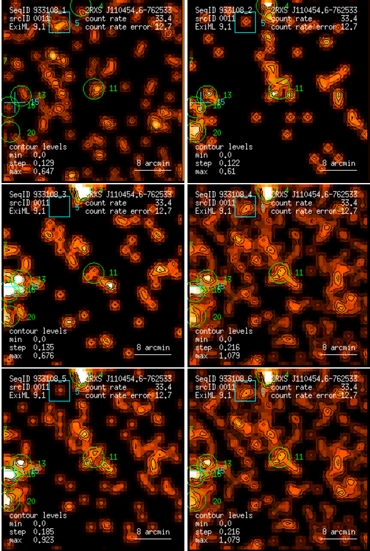
Figure 11: RASS 933108: detection 0011: band rate images, Gaussian filter: (1) PSPC channels 11 – 41, (2) 52 – 90, (3) 91 – 201, (4) 11 – 235, (5) 52 – 201, (6) 11 – 201. Broad band rates in counts/ks. Band rate contour levels in counts/ks/arcmin 2 .
