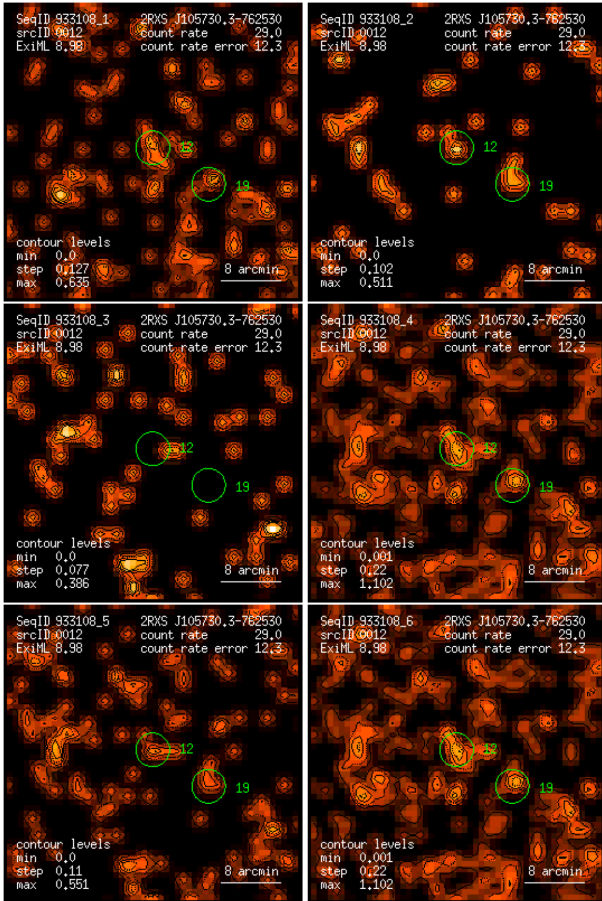
Figure 12: RASS 933108: detection 0012: band rate images, Gaussian filter: (1) PSPC channels 11 – 41, (2) 52 – 90, (3) 91 – 201, (4) 11 – 235, (5) 52 – 201, (6) 11 – 201. Broad band rates in counts/ks. Band rate contour levels in counts/ks/arcmin 2 .
